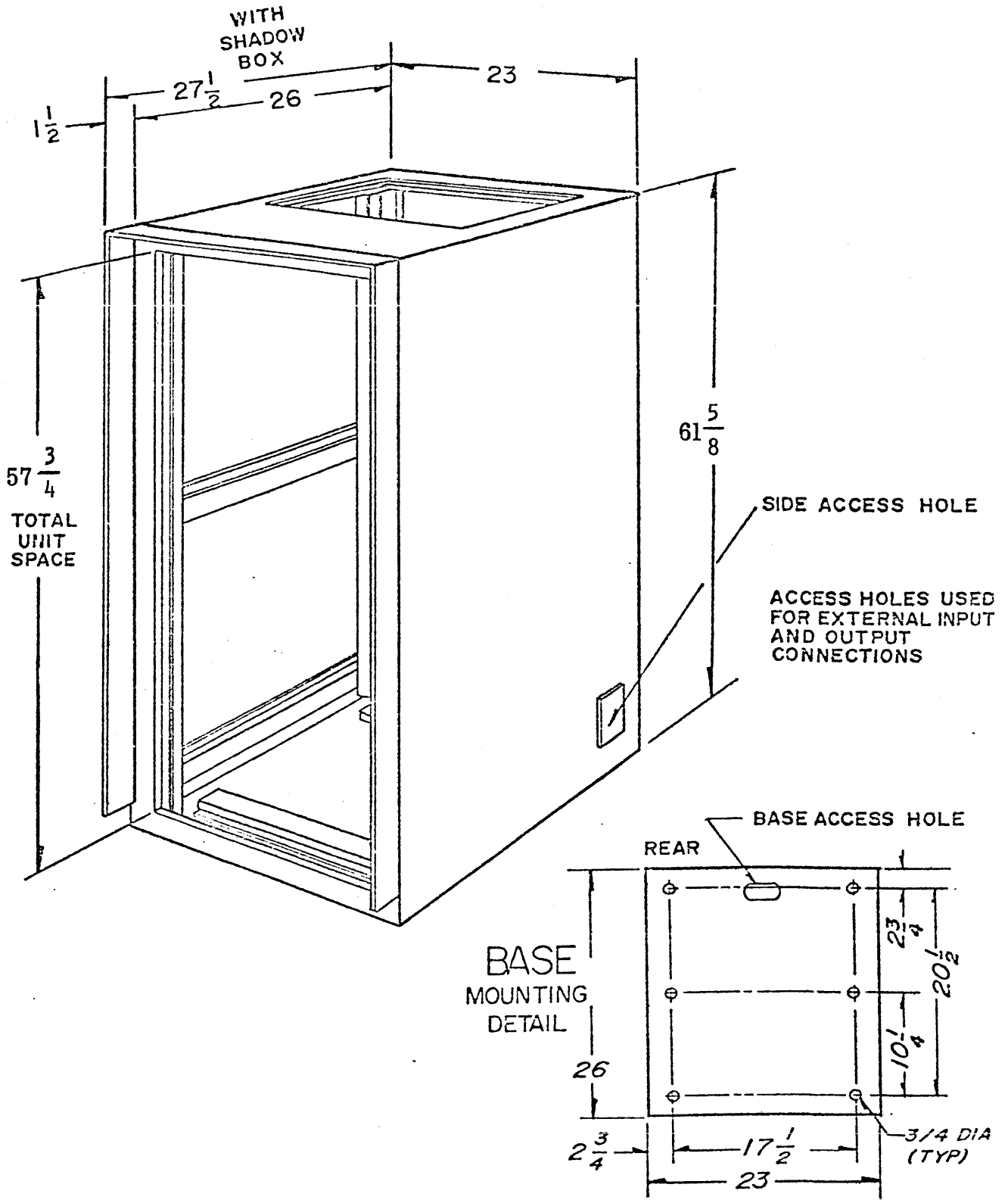
Figure 2-1. SYM3204A Cabinet Dimensions
