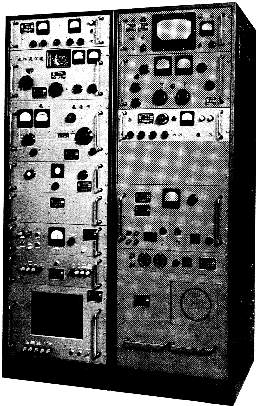
Figure I-1-1-b. Front View of Sideband Generator in Relation to SBT-1K Transmitter
