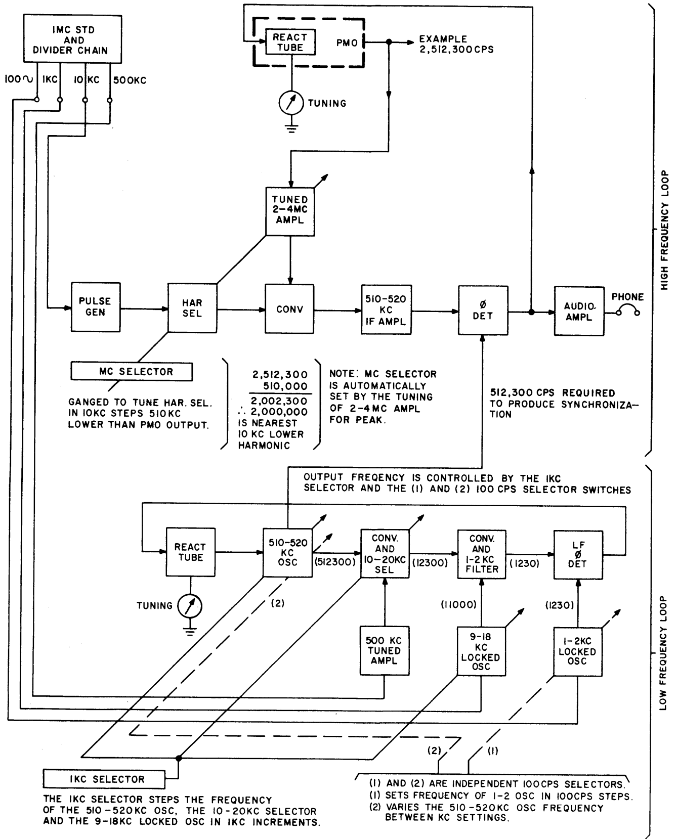
Figure I-4-3. Block Diagram Illustrating Frequency Translation in High Frequency and Low Frequency Loops
