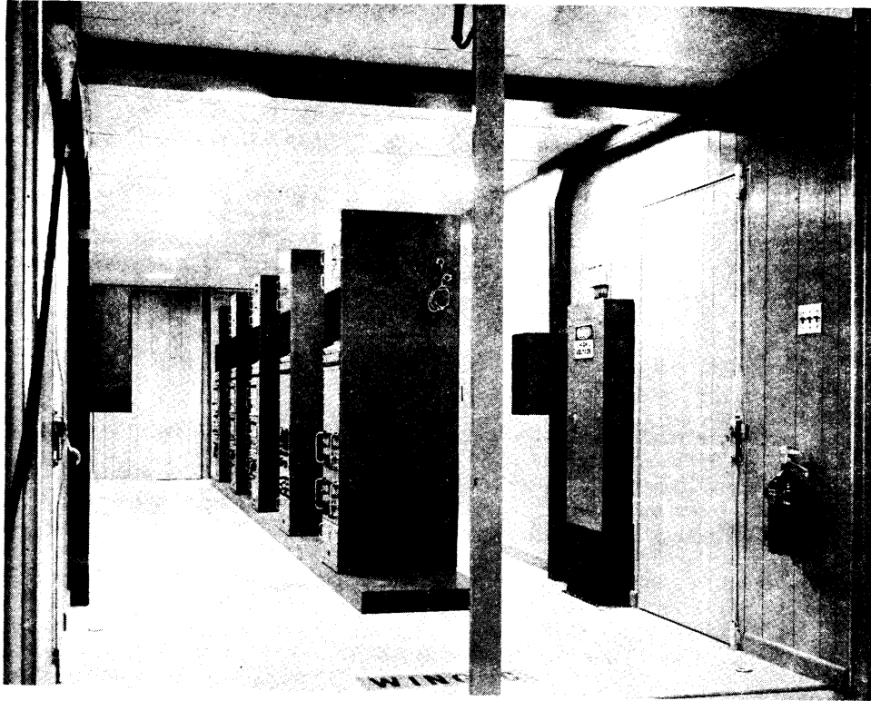
Figure 1-16. Receiving Central Group OA-4939/TSR-1 (RC1, Equipment Installation)
