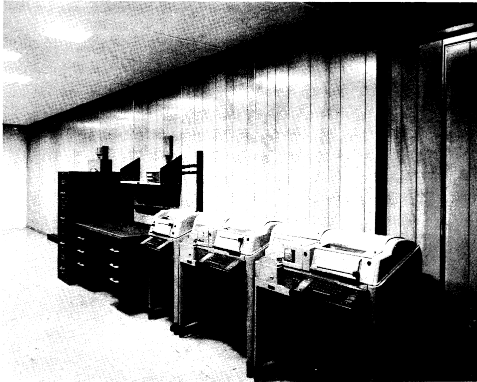
Figure 1-29. Control Monitor Group OA-4950/TSR-1 (RF2, Right Side Equipment)
