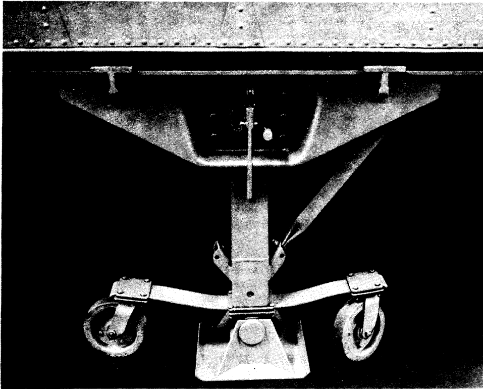
Figure 1-58. Container Support Assembly
