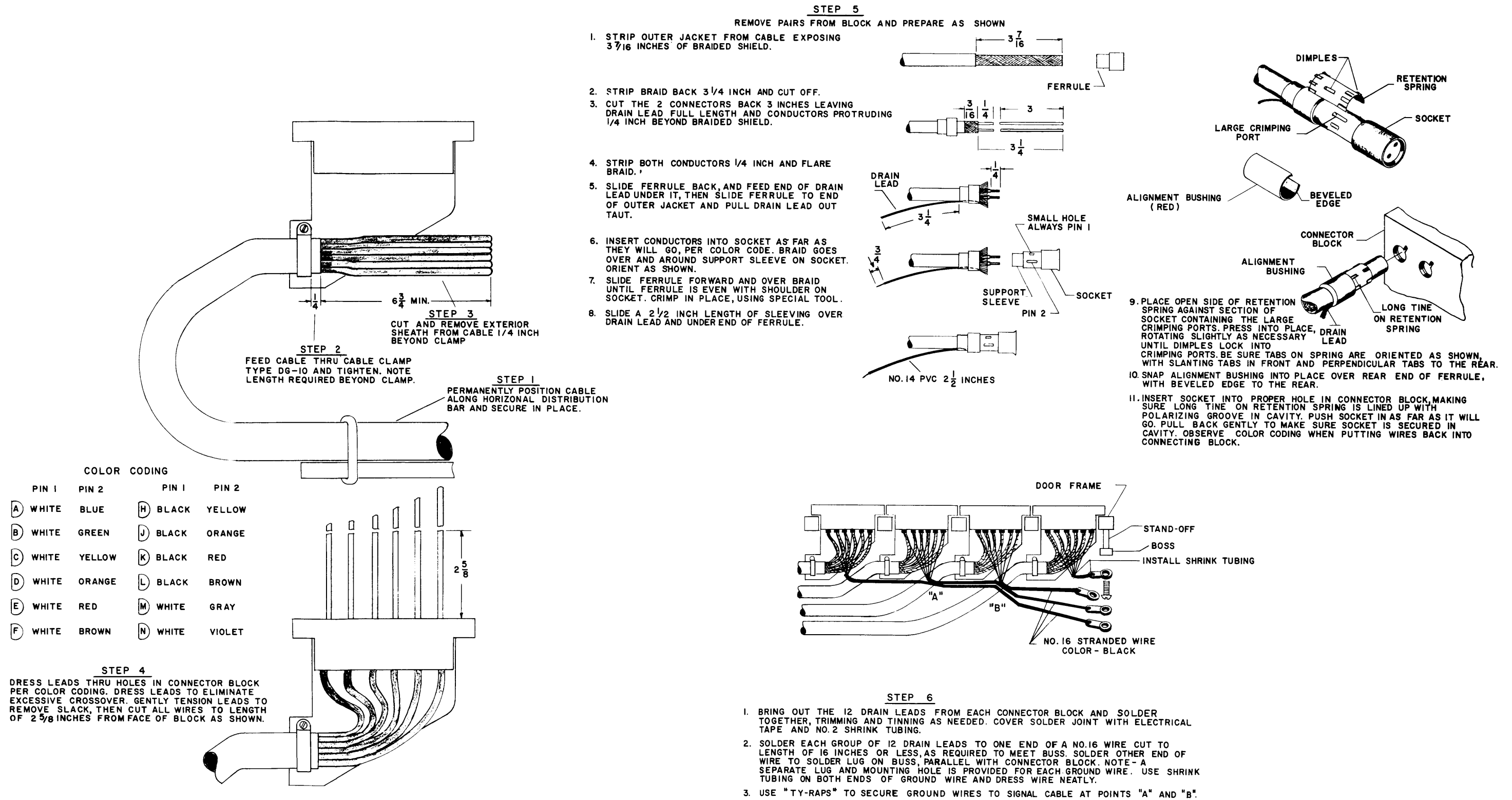
Figure 2-3. Wiring Standard MDF Block Cable Termination
