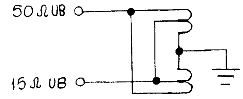
SCHEMATIC DIAGRAM
