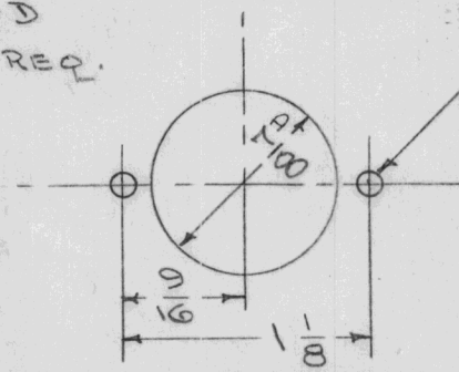
DRILLING PLAN
