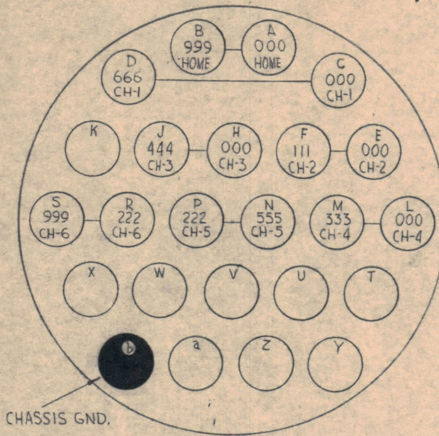
24 PIN RECEPTACLE AMPHENOL -67-02E18-24P
