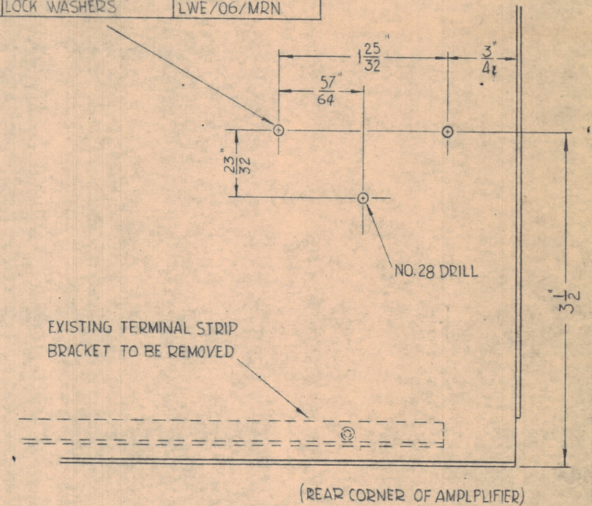
DRILLING LAYOUT VOYCALL AMPLIFIER
