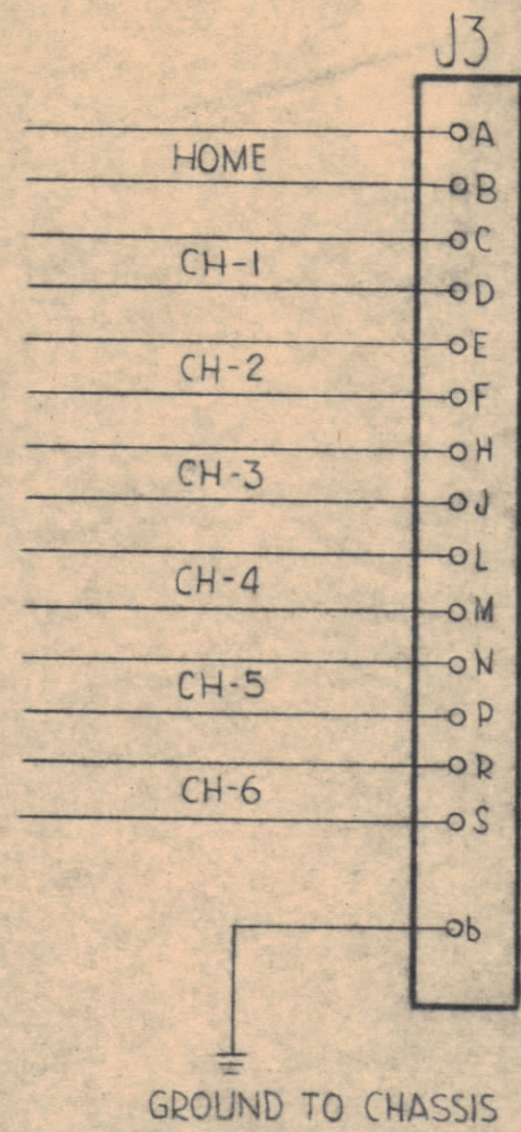
J3-24 PIN CONNECTOR AMPHENOL -67-02E18-24P
