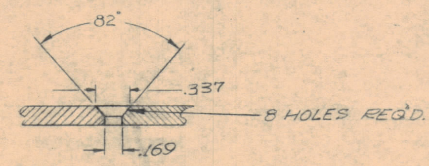
DETAIL - C
