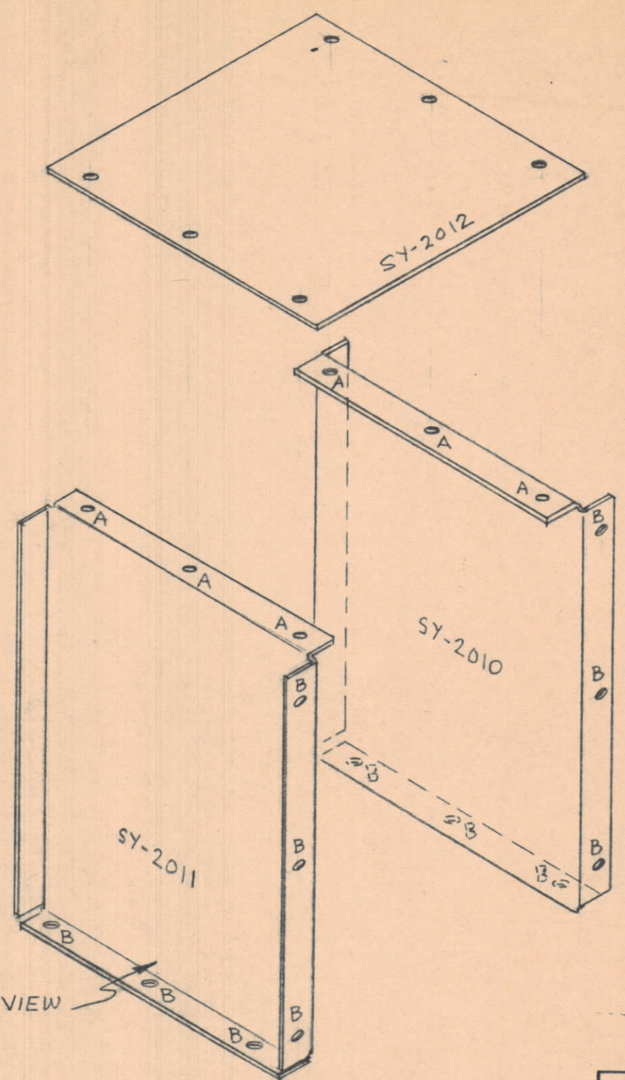
ISOMETRIC VIEW
