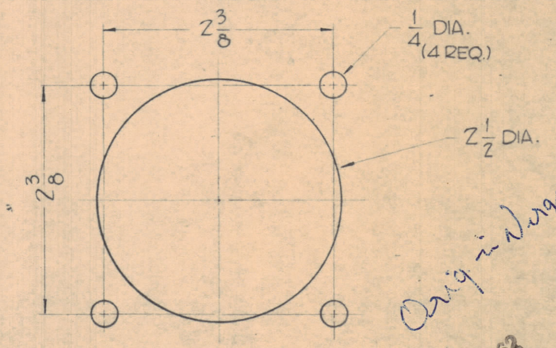
DETAIL "C" (1 REQ.)
