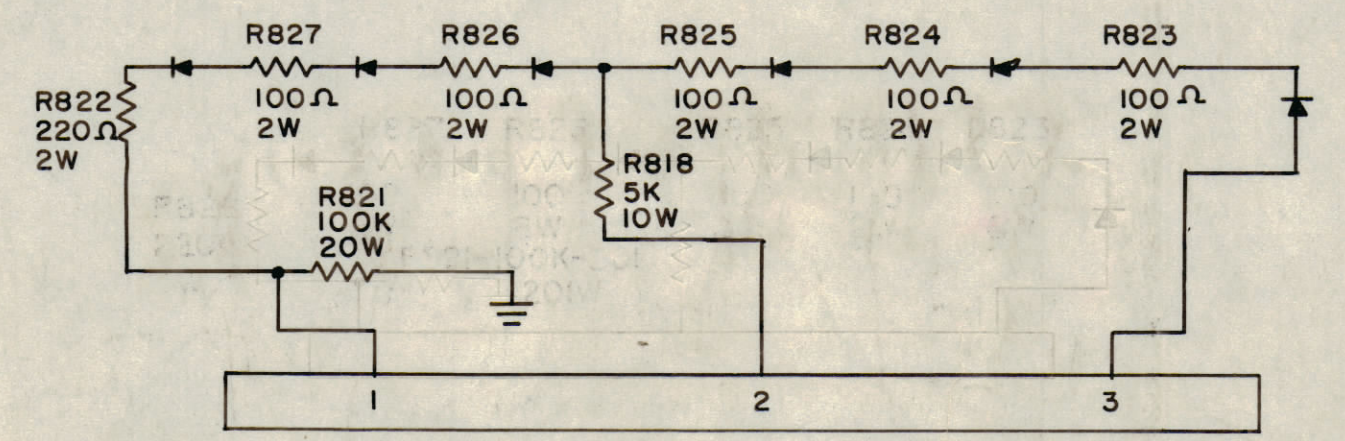
SCHEMATIC FIGURE 3
