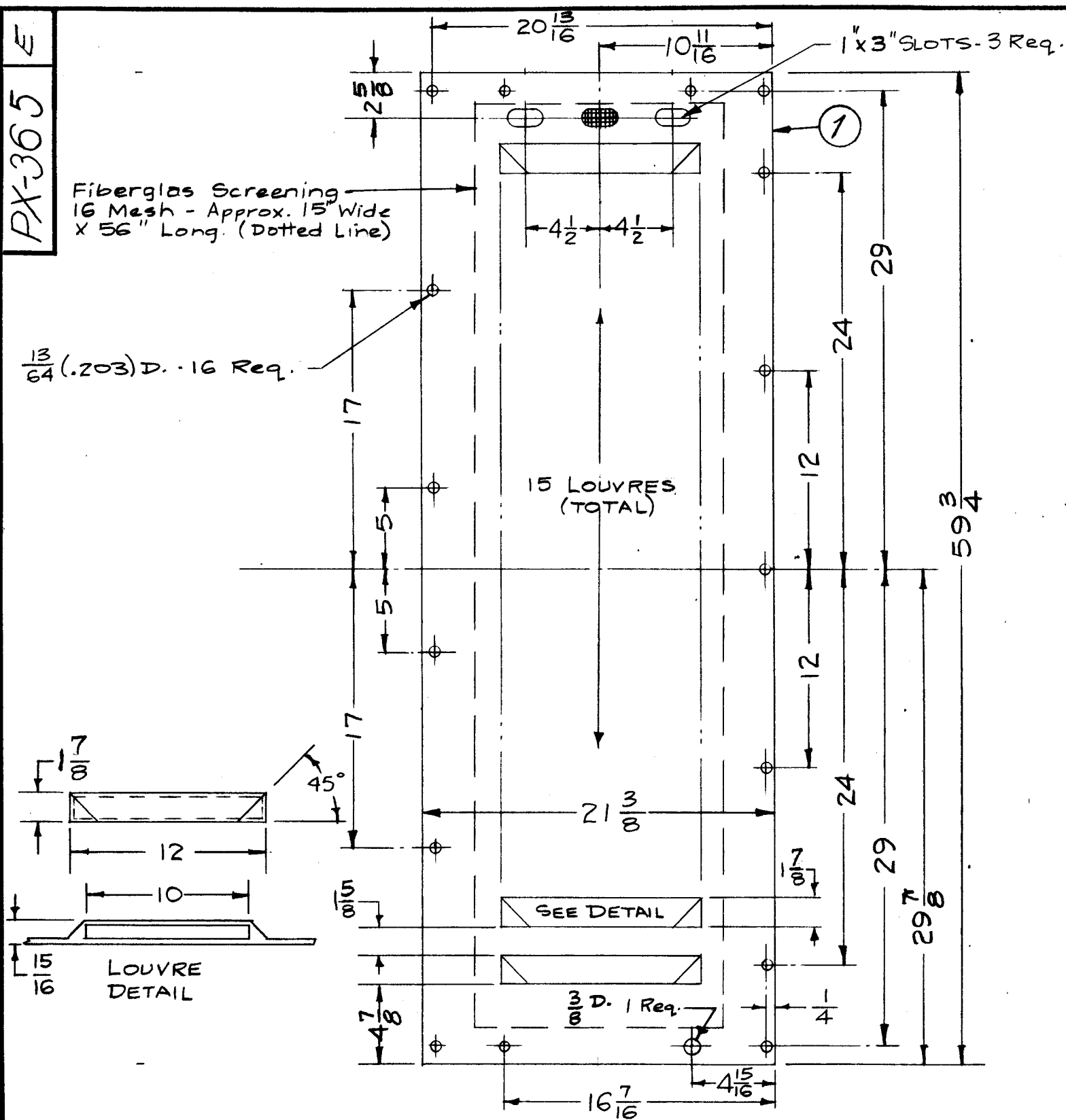
PX-365-1 PANEL, REAR, LEFT
