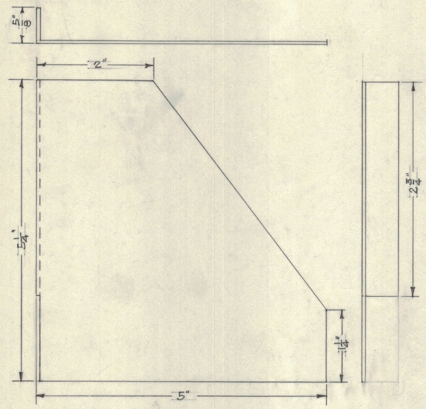
LEFT SUPPORT BRACKET
