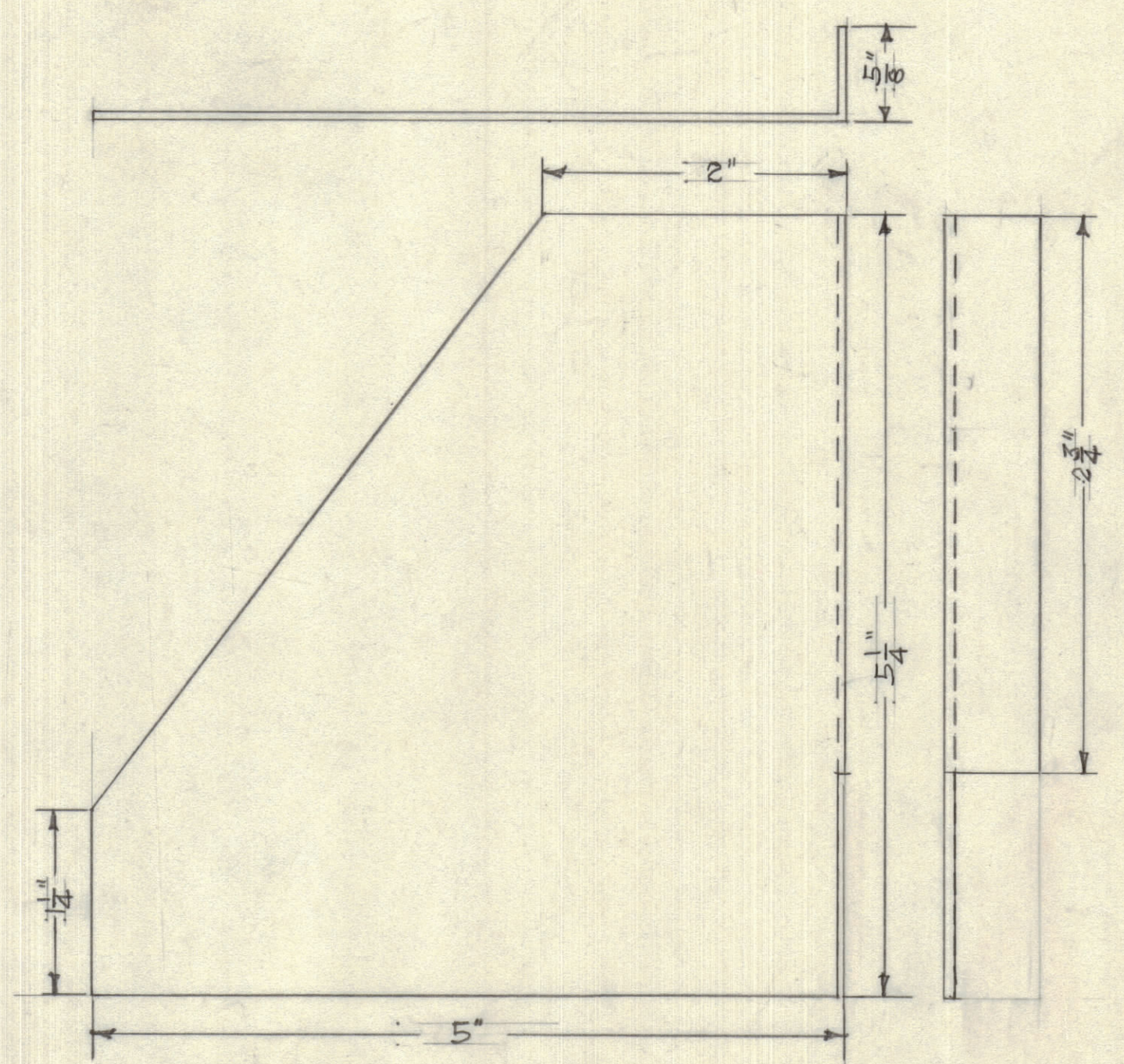
RIGHT SUPPORT BRACKET
