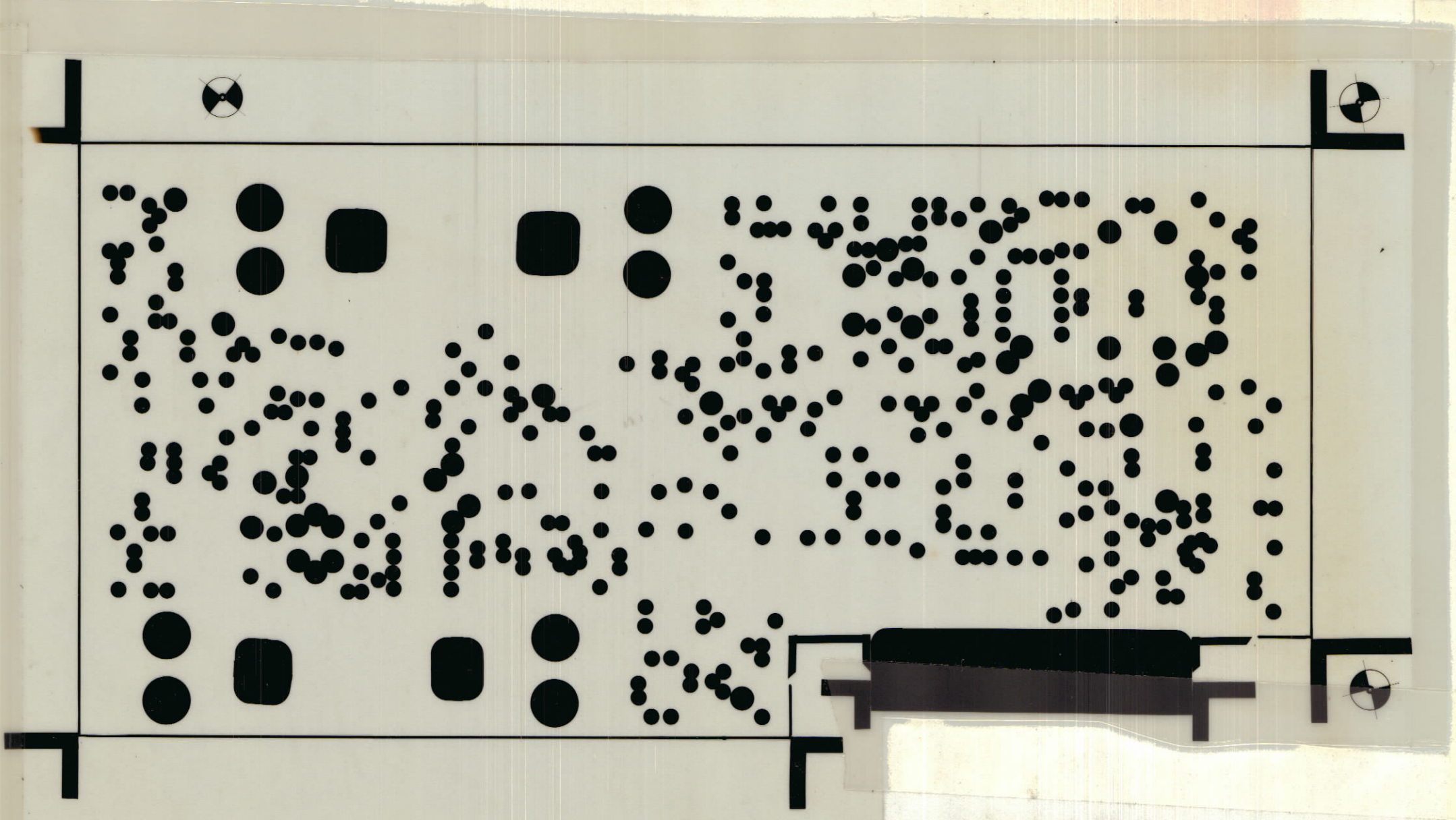
SOLDER MASK PC825-5 (CIRCUIT SIDE)
