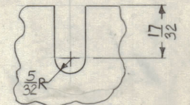
"B" DETAIL 2 REQ.
