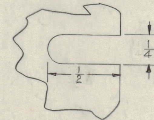
SLOT "F" DETAIL 4 Req'd.
