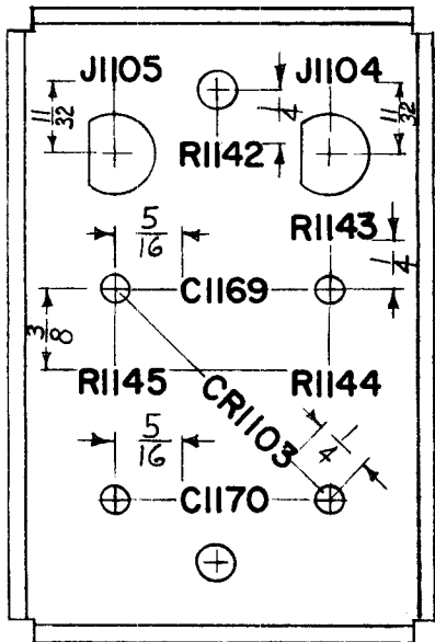
BOTTOM VIEW
