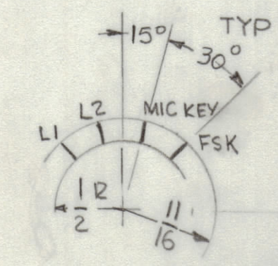
TYPICAL FOR LSB & USB
