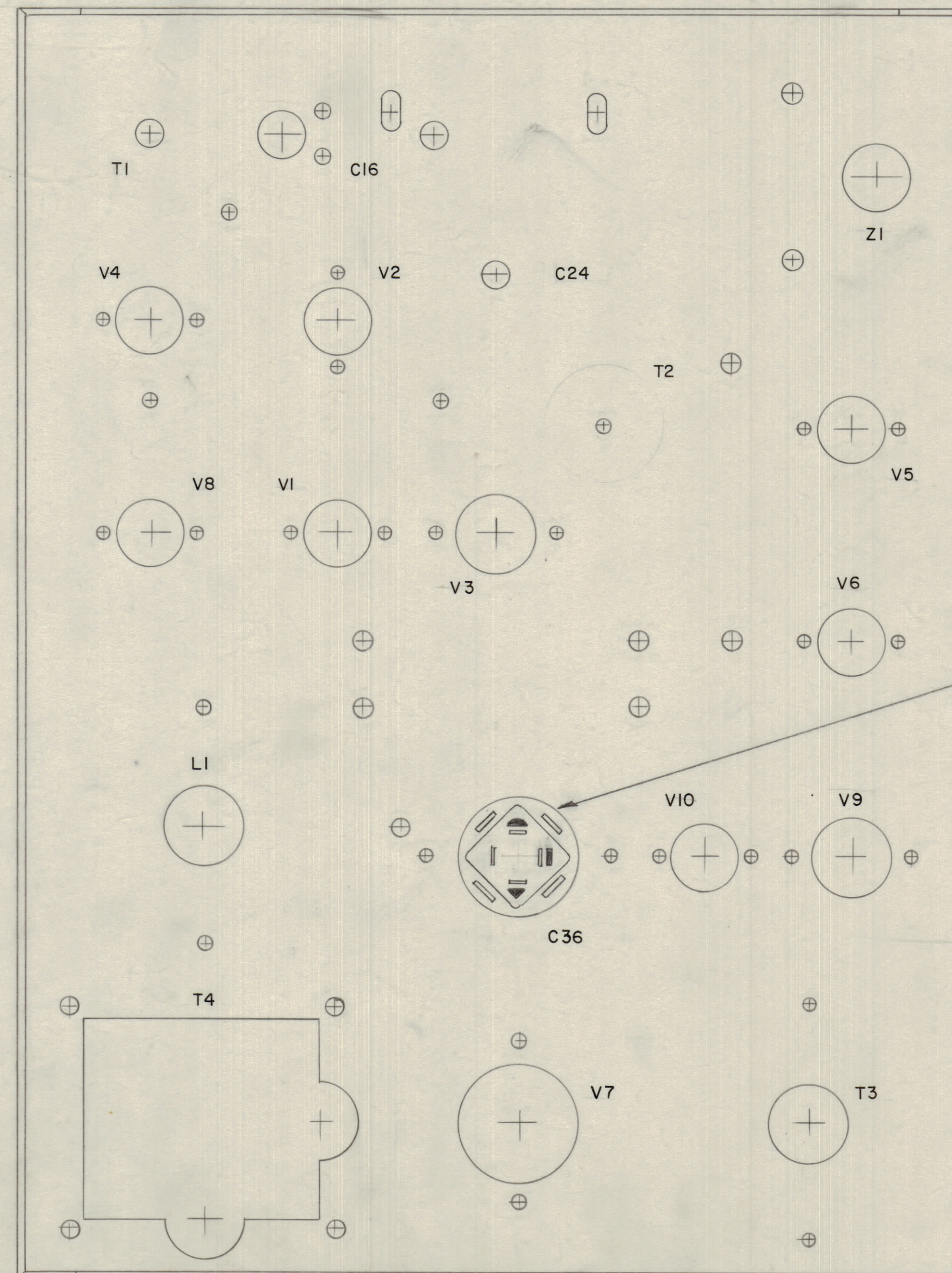
BOTTOM VIEW, INSIDE
