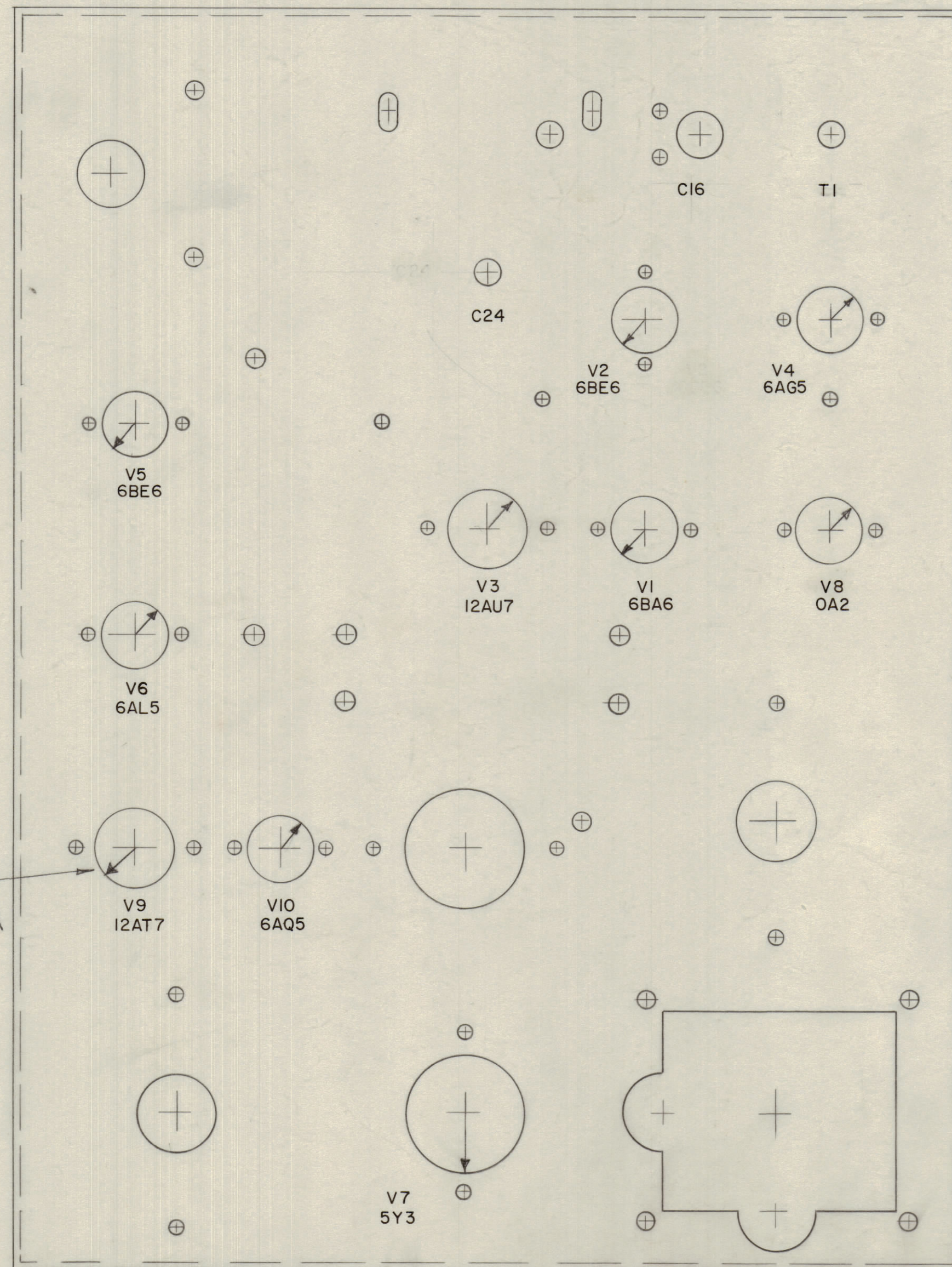
TOP VIEW, OUTSIDE
