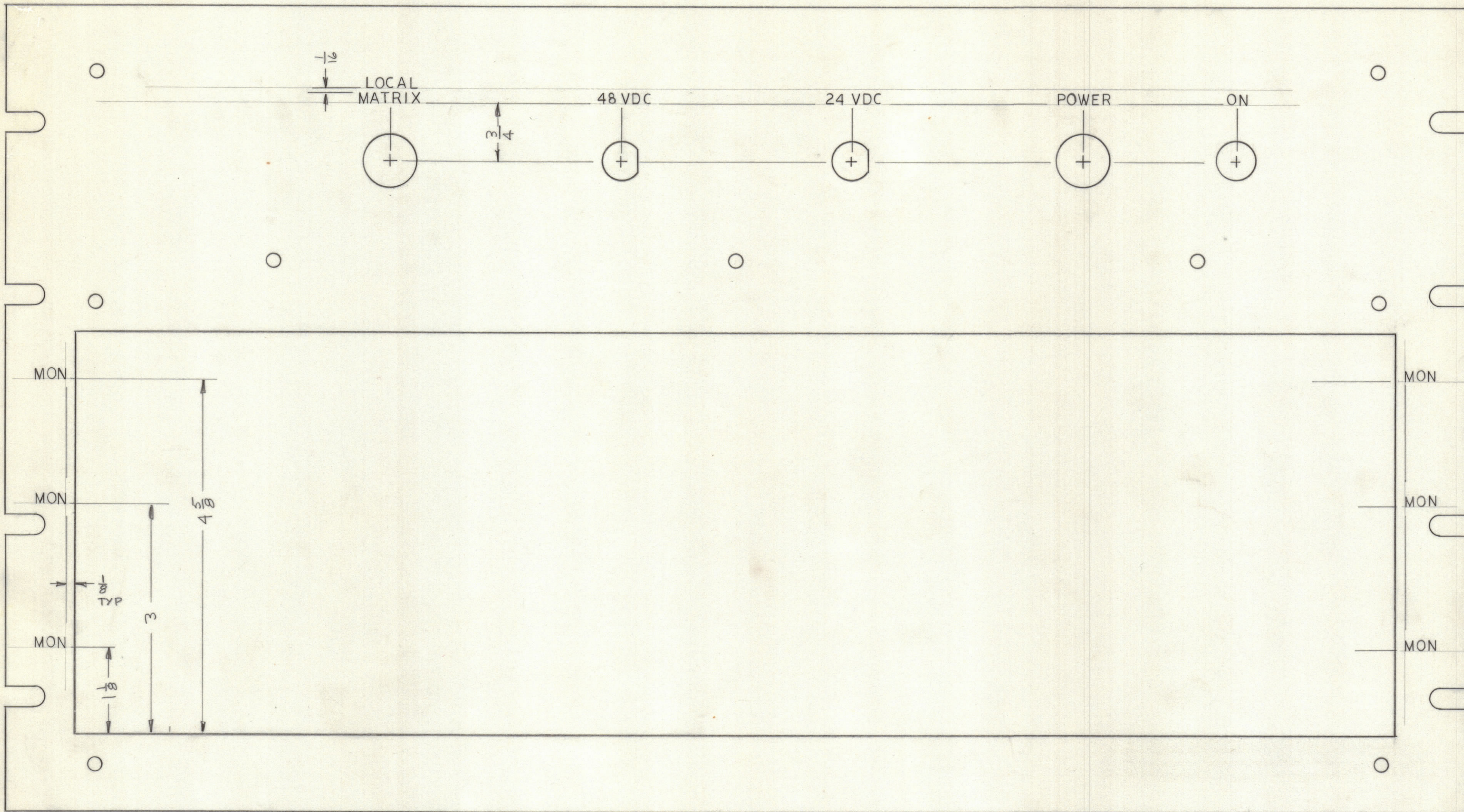
ENGRAVING - FRONT VIEW
