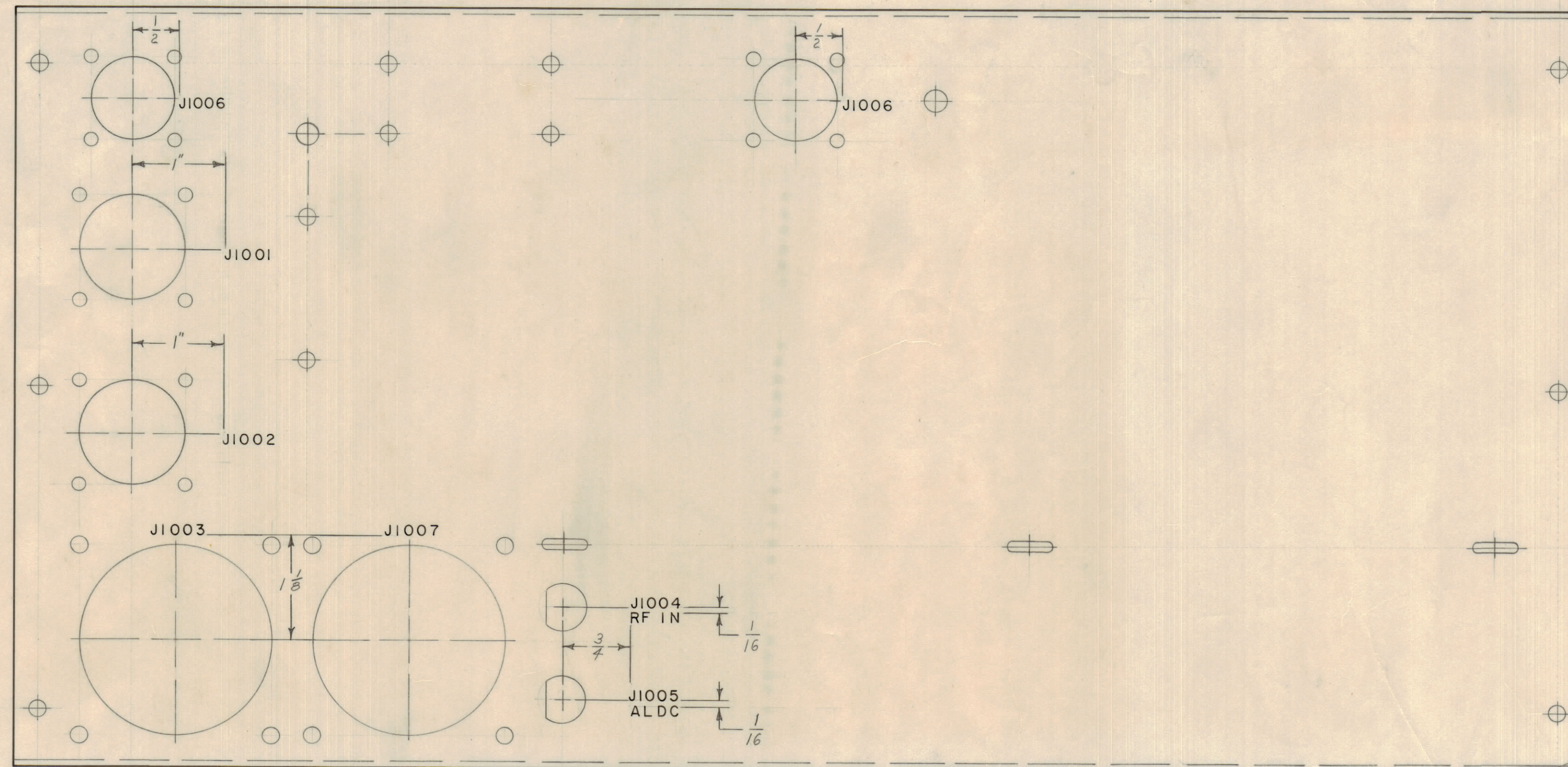
OUTSIDE VIEW
