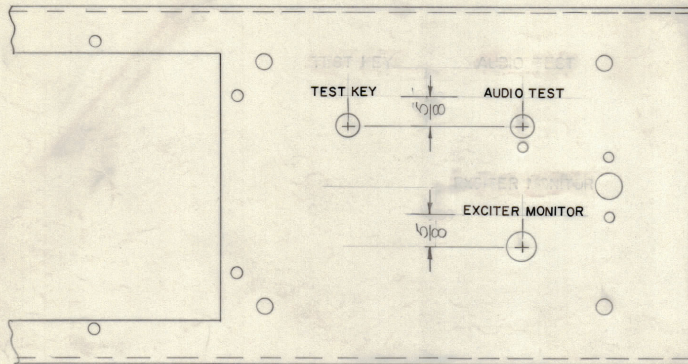
ENGRAVING FRONT VIEW
