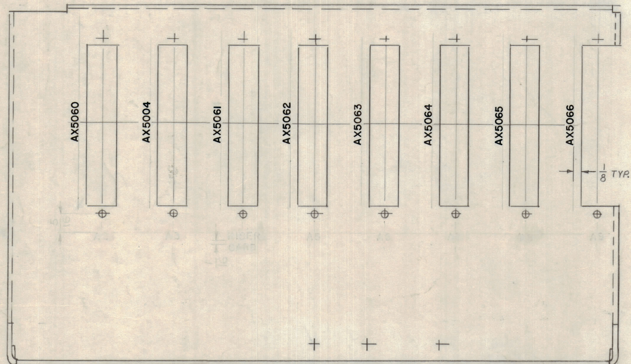
TOP VIEW
