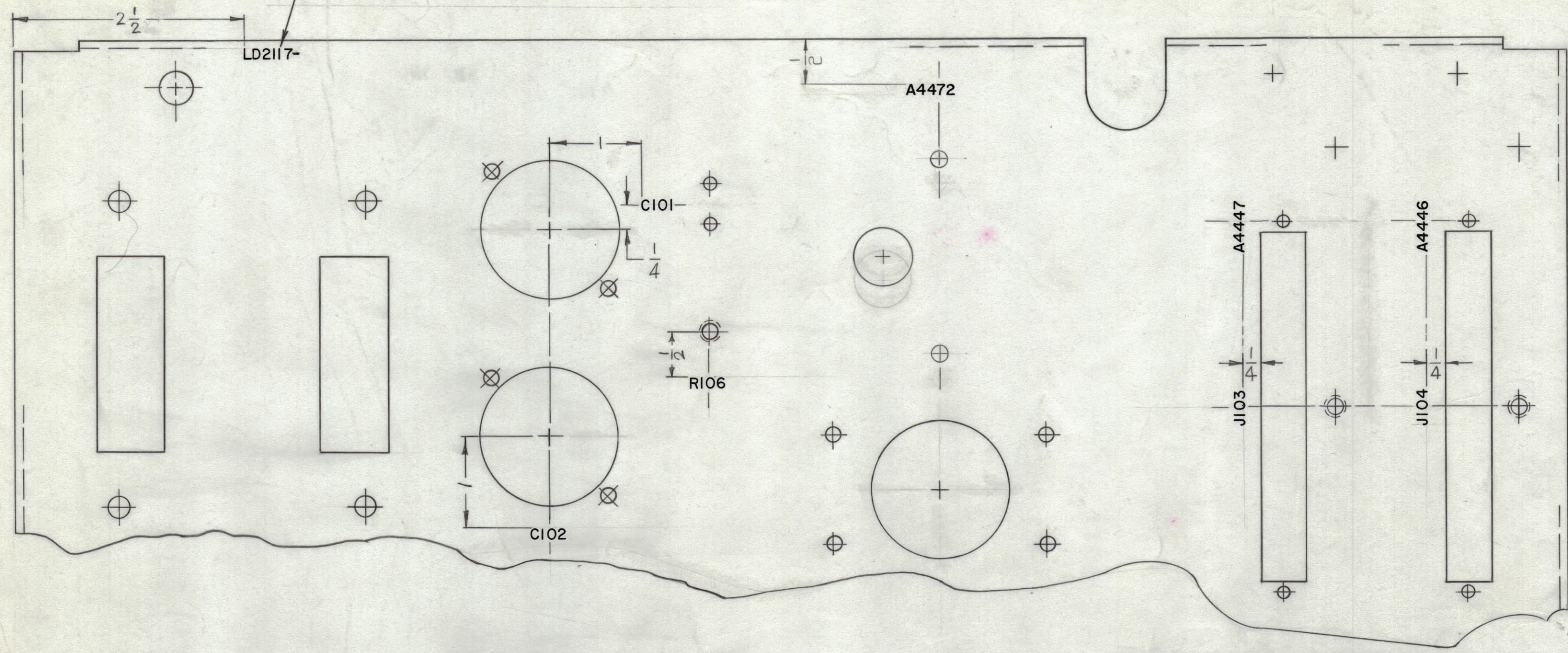
TOP VIEW OF CHASSIS SHOWN
