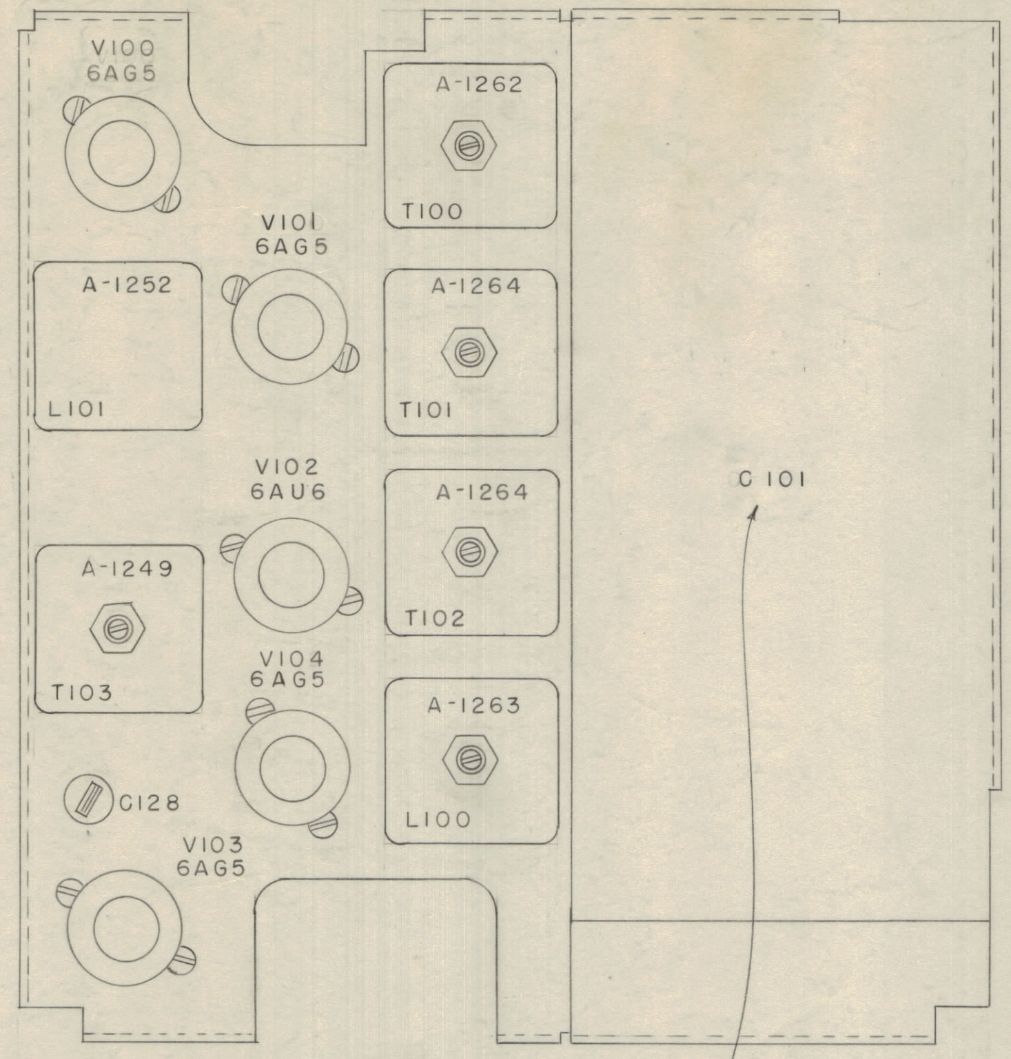
CHASSIS TOP
