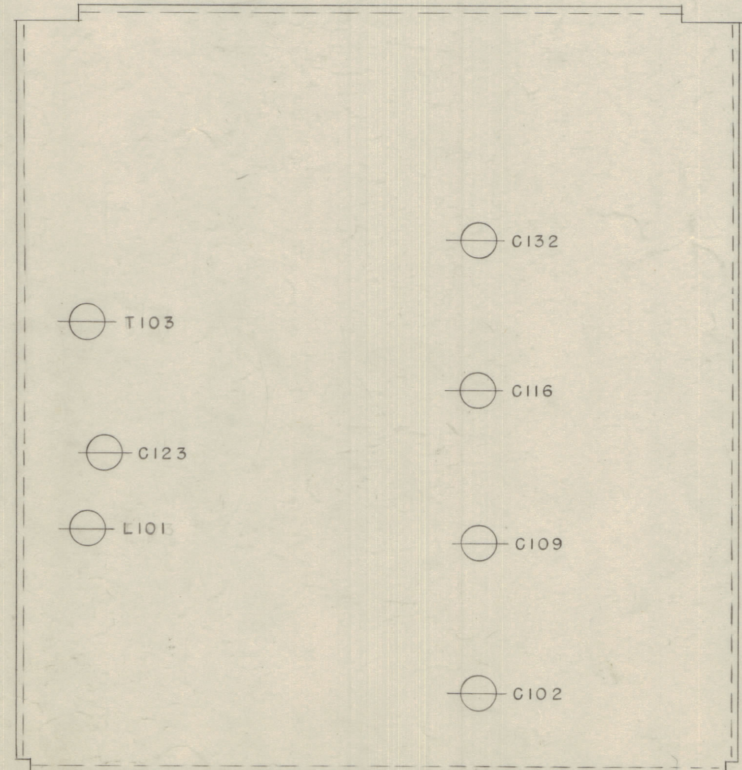
BOTTOM COVER
