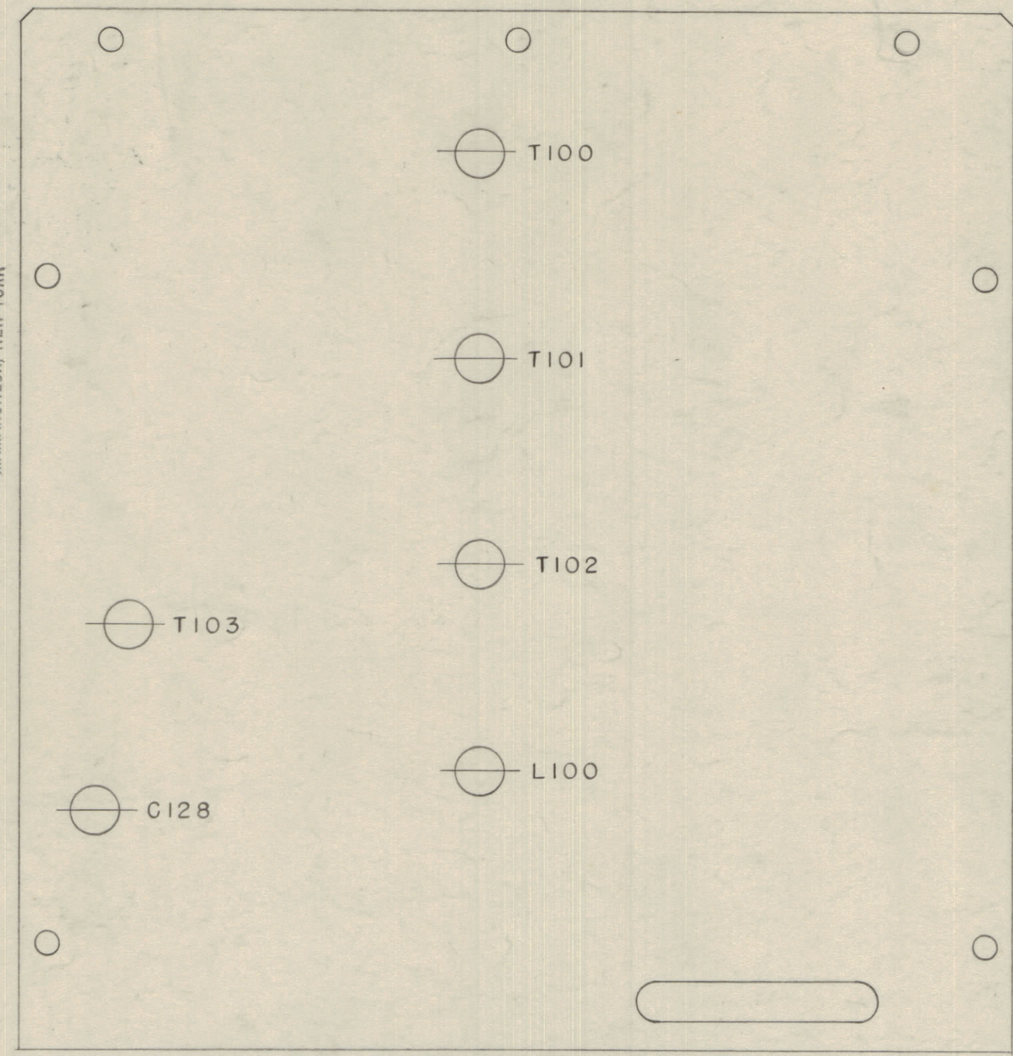
TOP COVER
