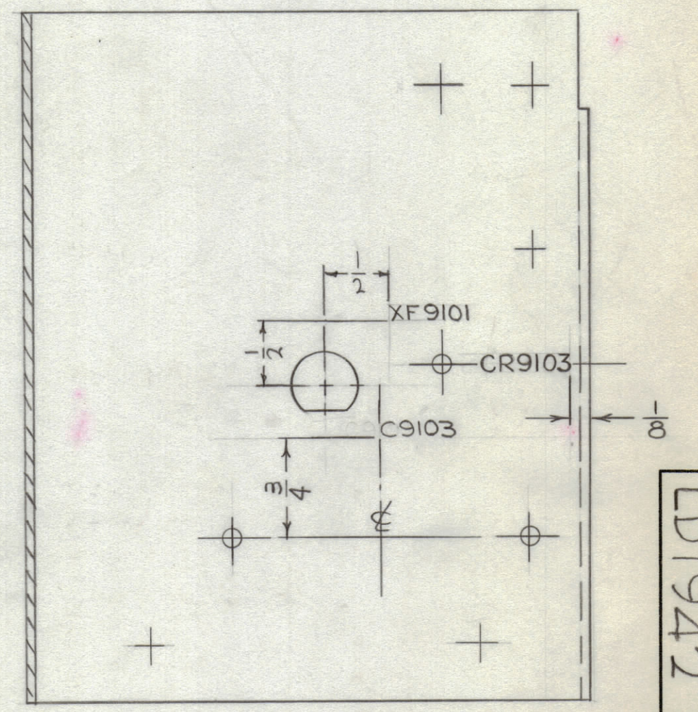
VIEW "B-B"
