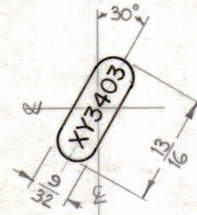
TYP. CRYSTAL LAYOUT
