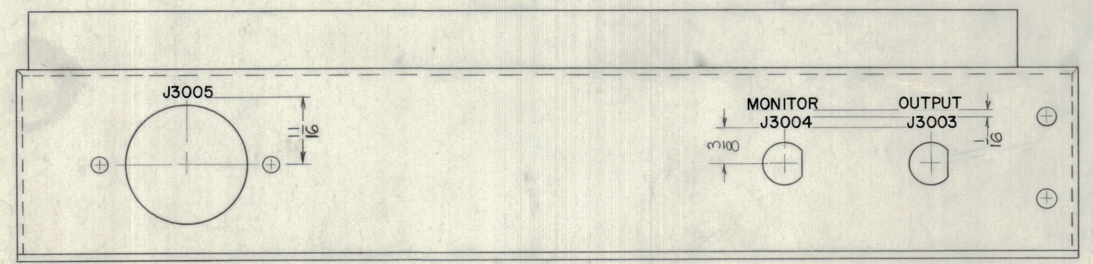
- TOP VIEW -
