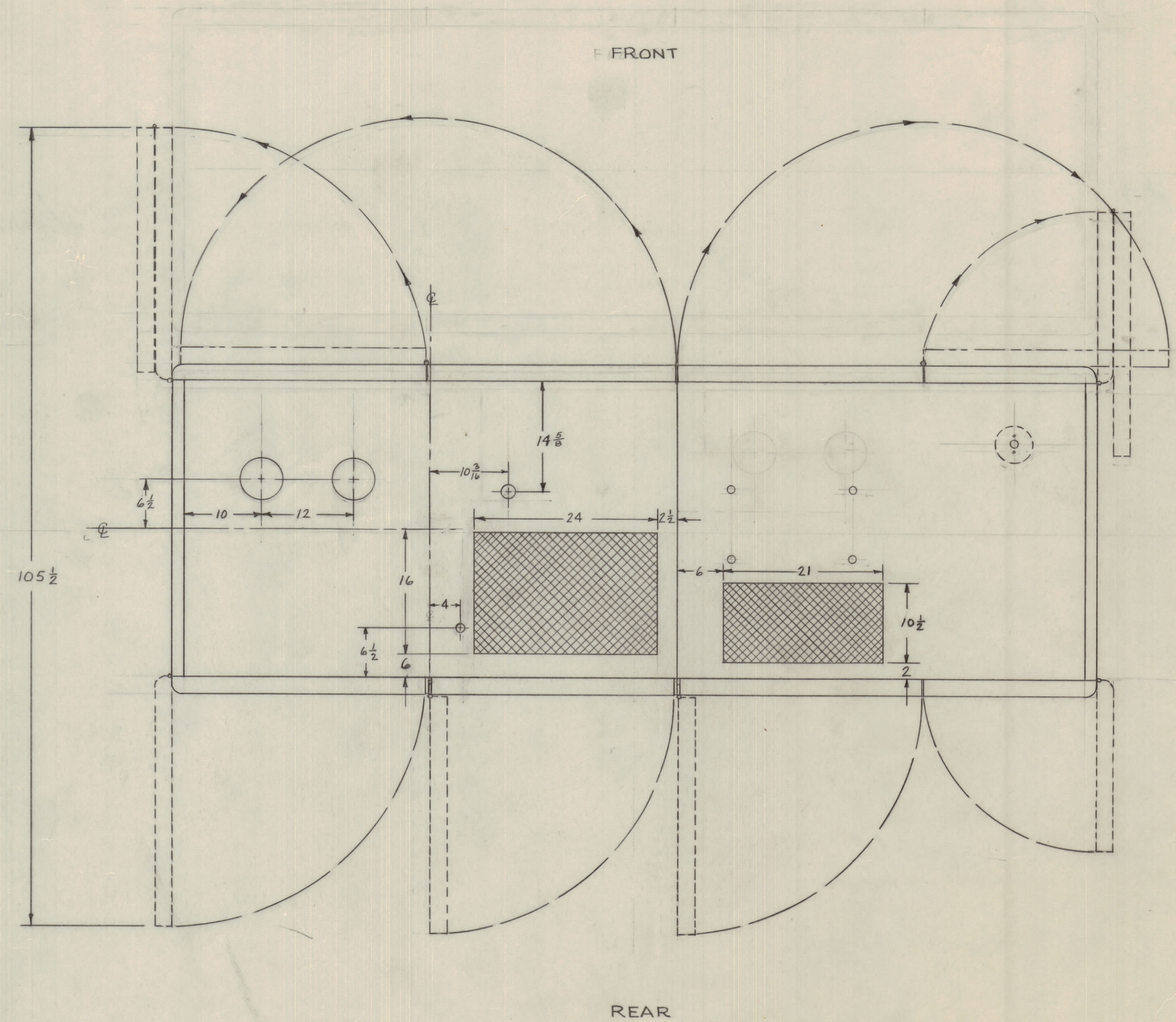
PLAN DETAIL OF TOP COVER AND DOOR CLEARANCE
