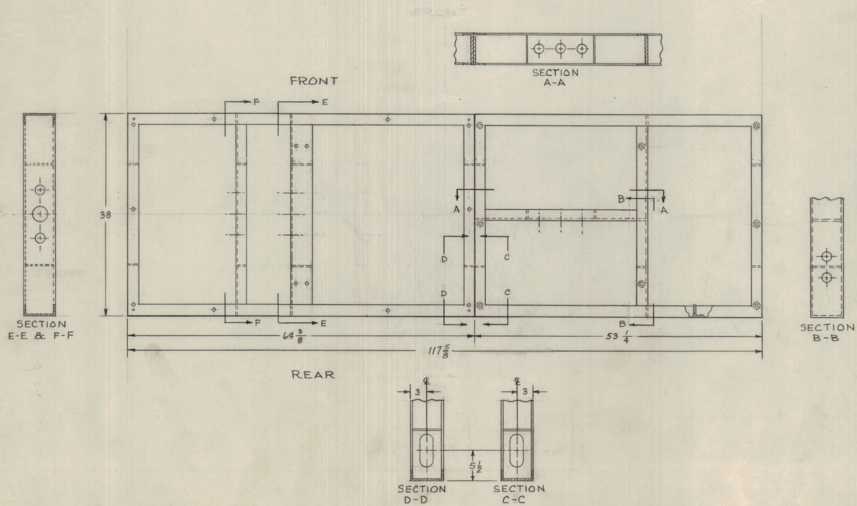
PLAN DETAIL OF BASE
