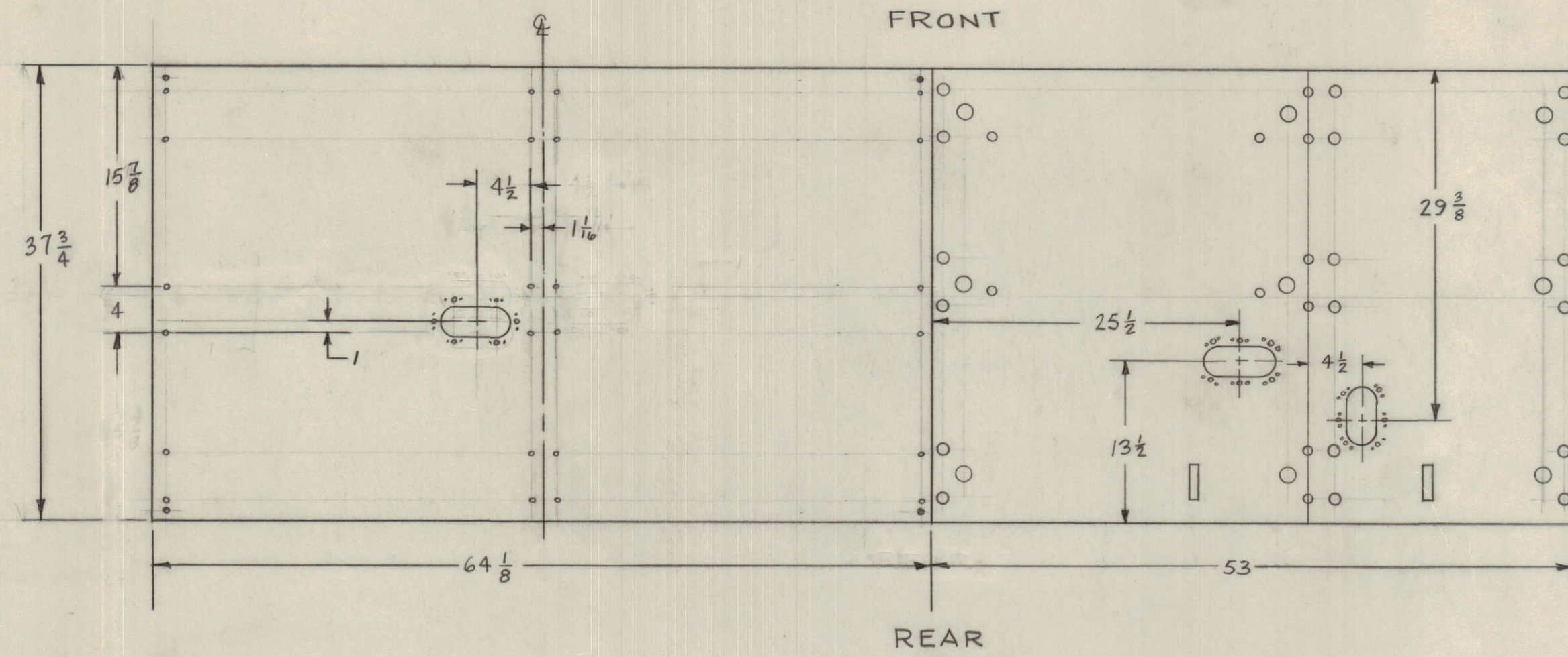
PLAN DETAIL OF BASE SHIELDS
