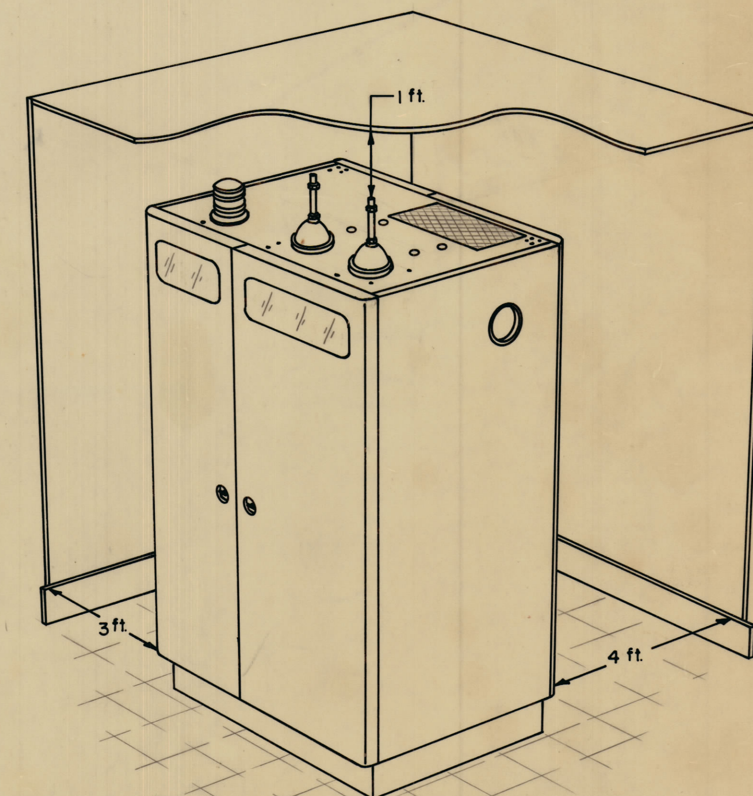
RECOMMENDED MINIMUM CLEARANCE REQUIREMENTS
