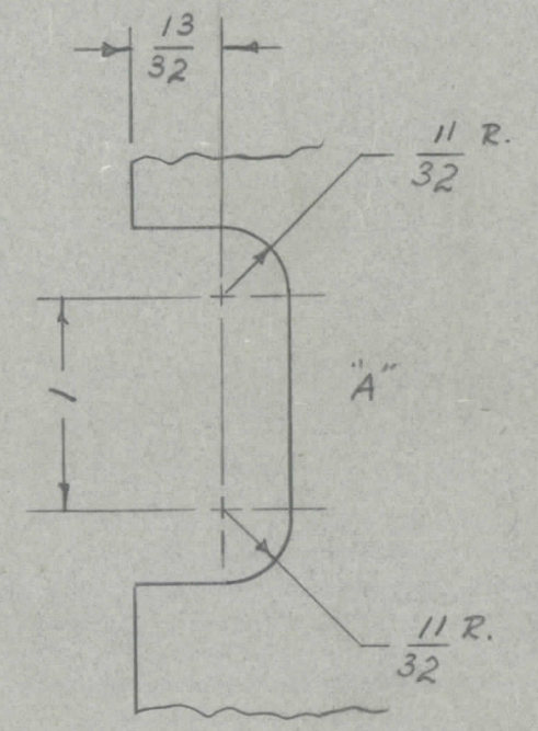
DETAIL "A"
