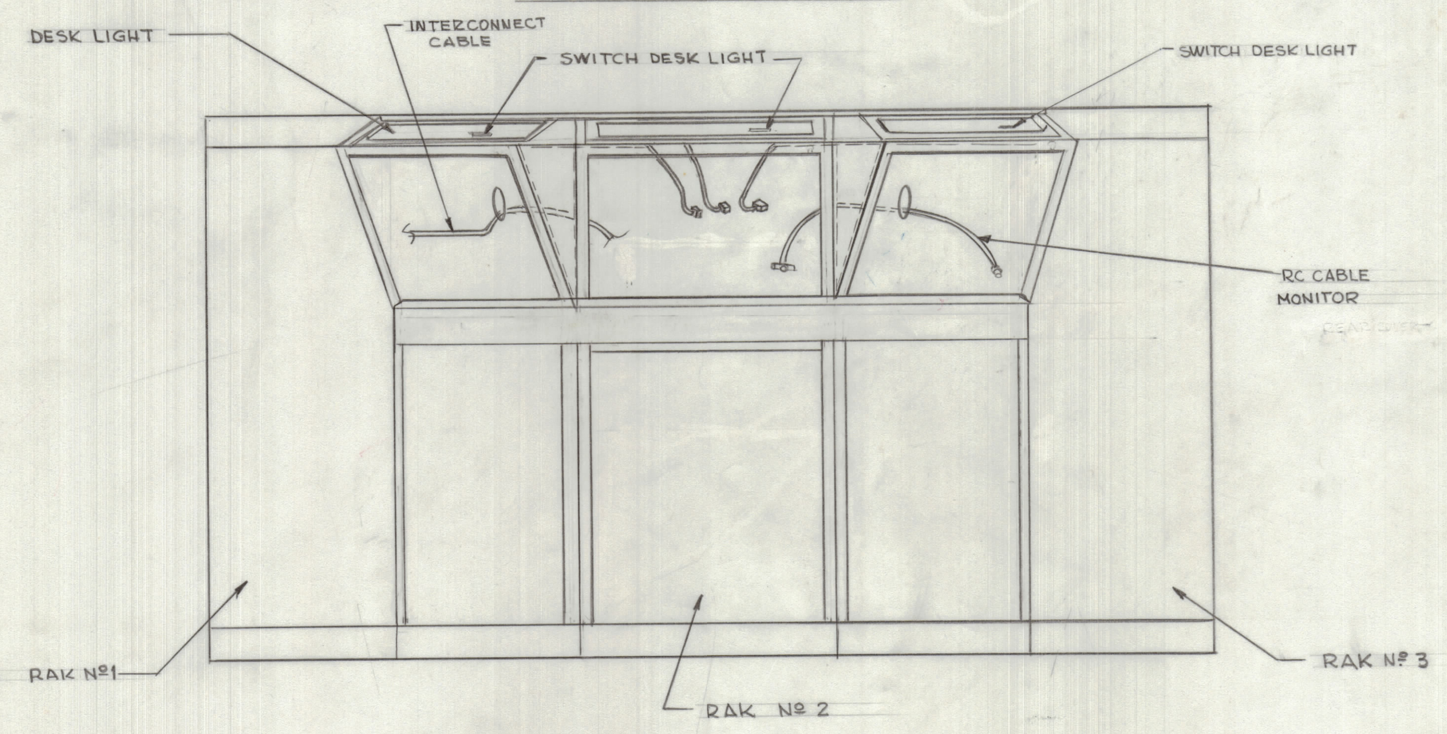
FRONT VIEW
