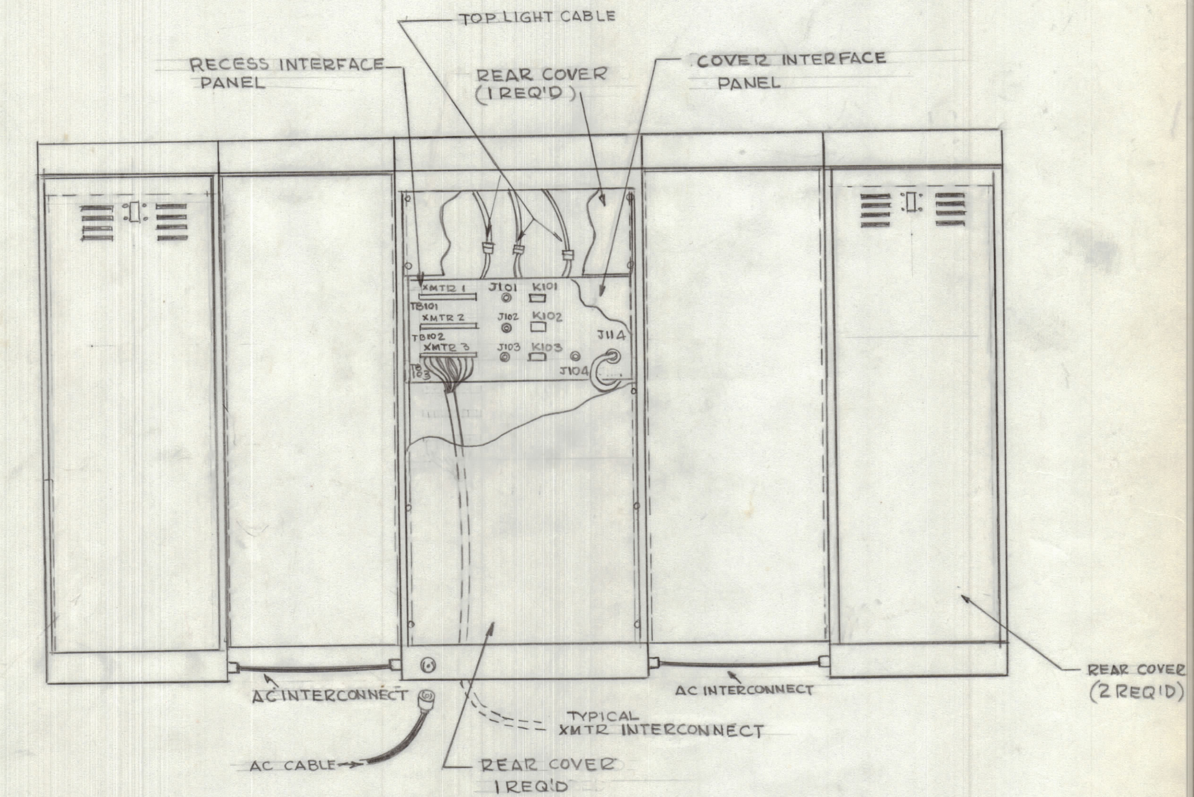
REAR VIEW
