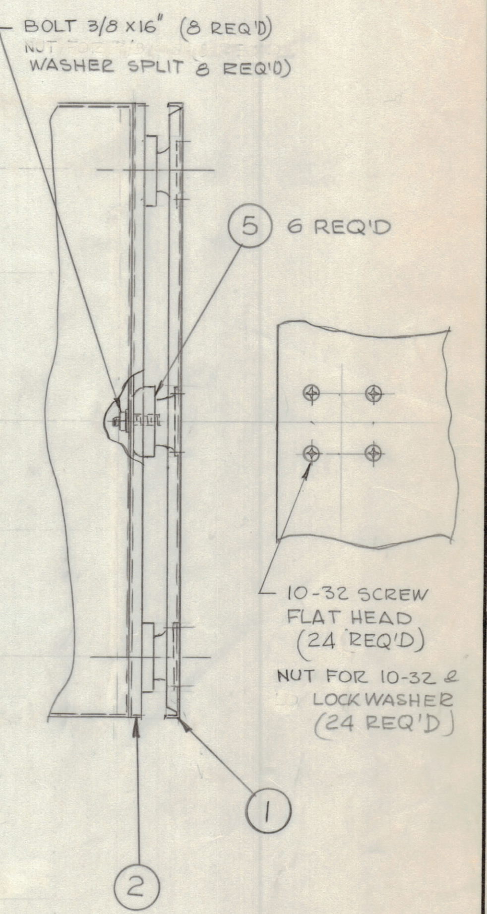
FLOOR DRILLING DETAIL
