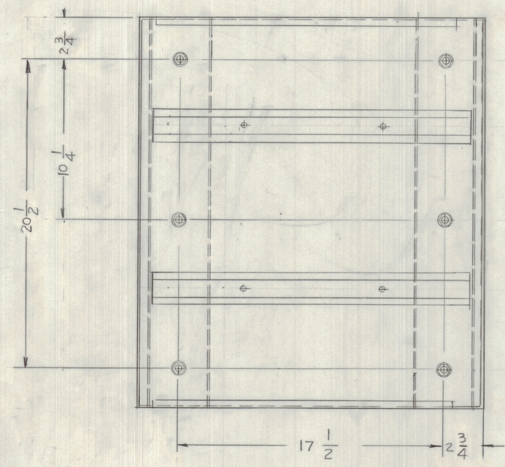
FLOOR DRILLING DETAIL
