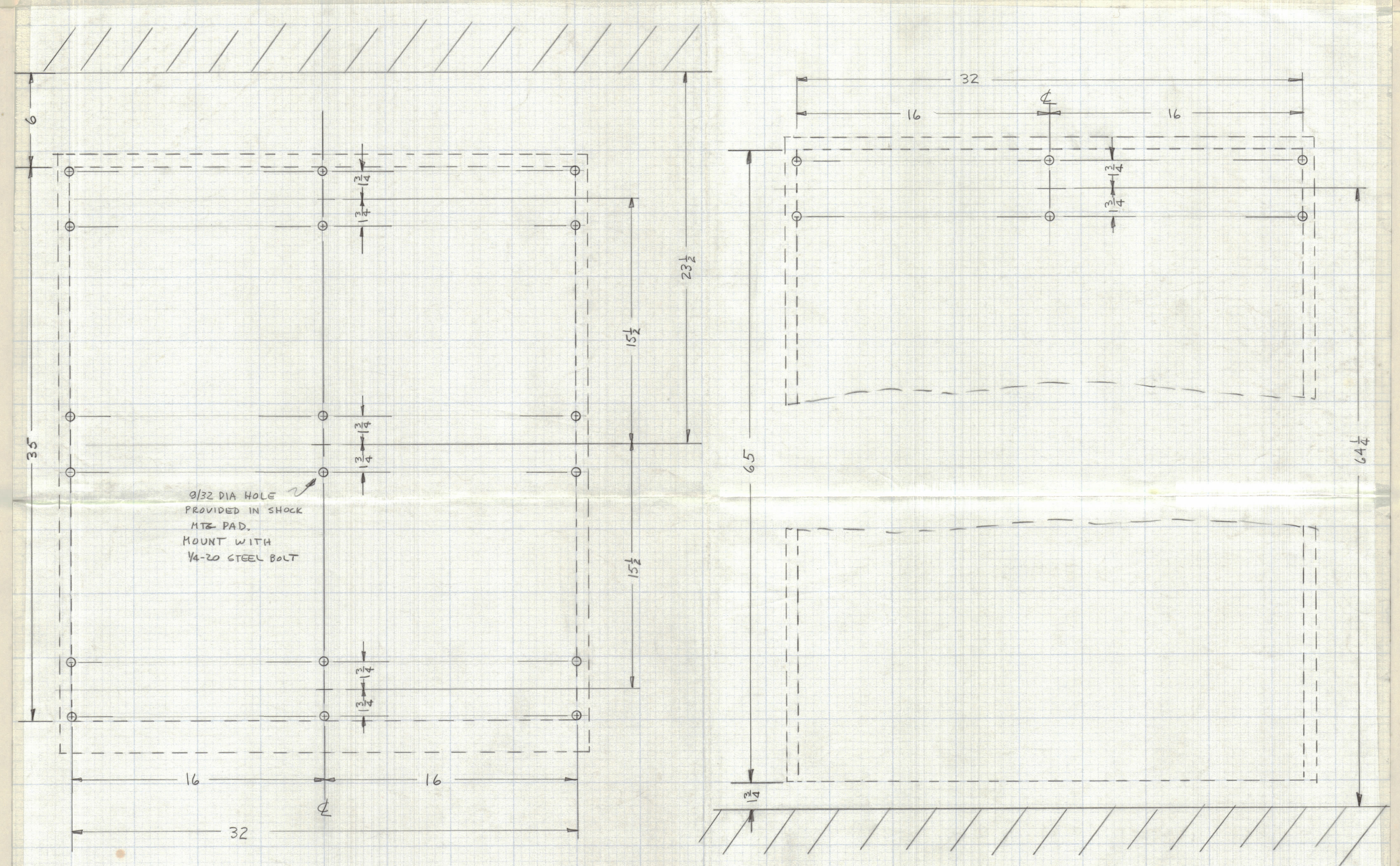
FLOOR HOLE LAYOUT HFT(-)10K SHOCK MTB
