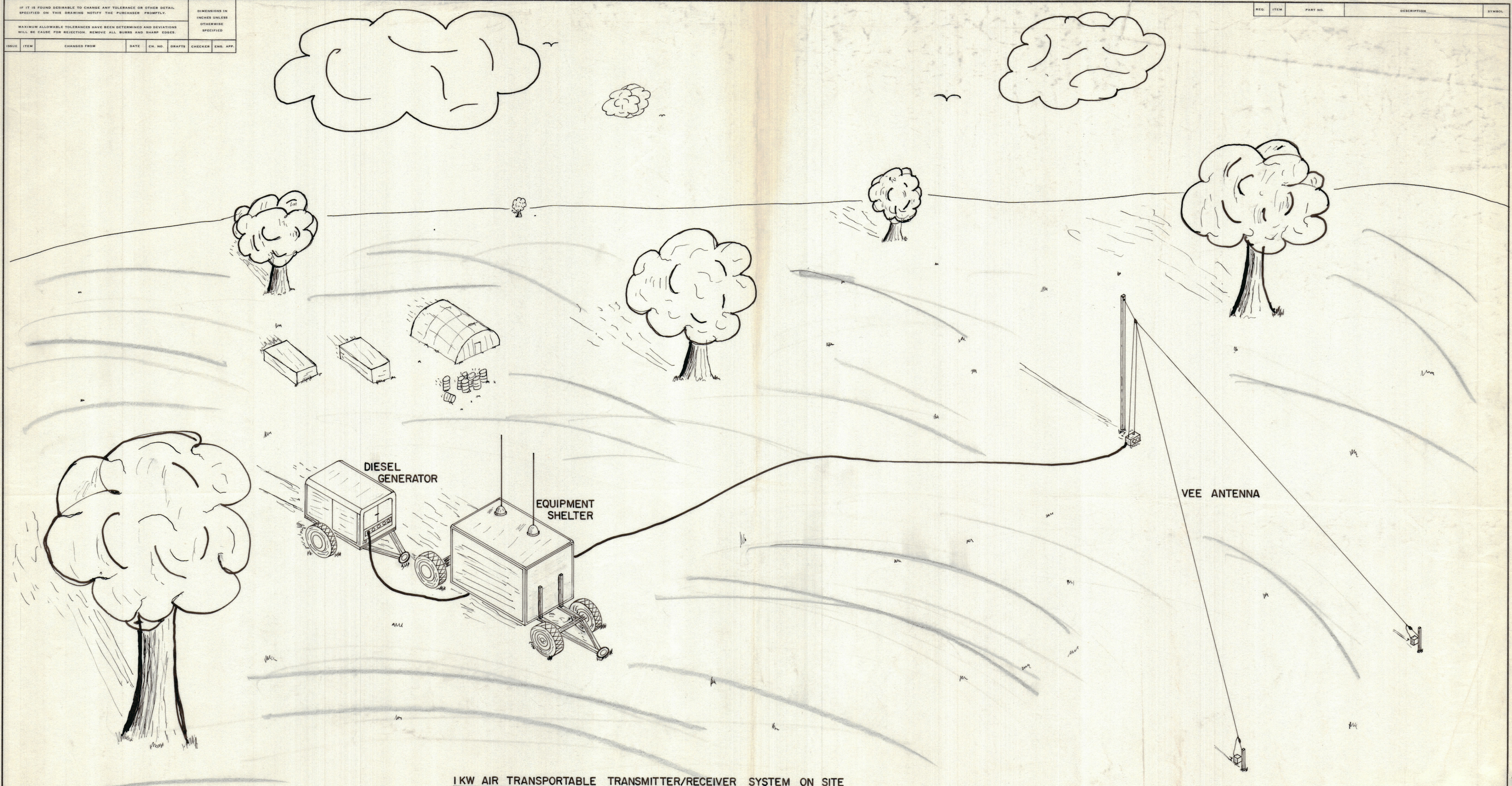
IKW AIR TRANSPORTABLE TRANSMITTER/RECEIVER SYSTEM ON SITE
