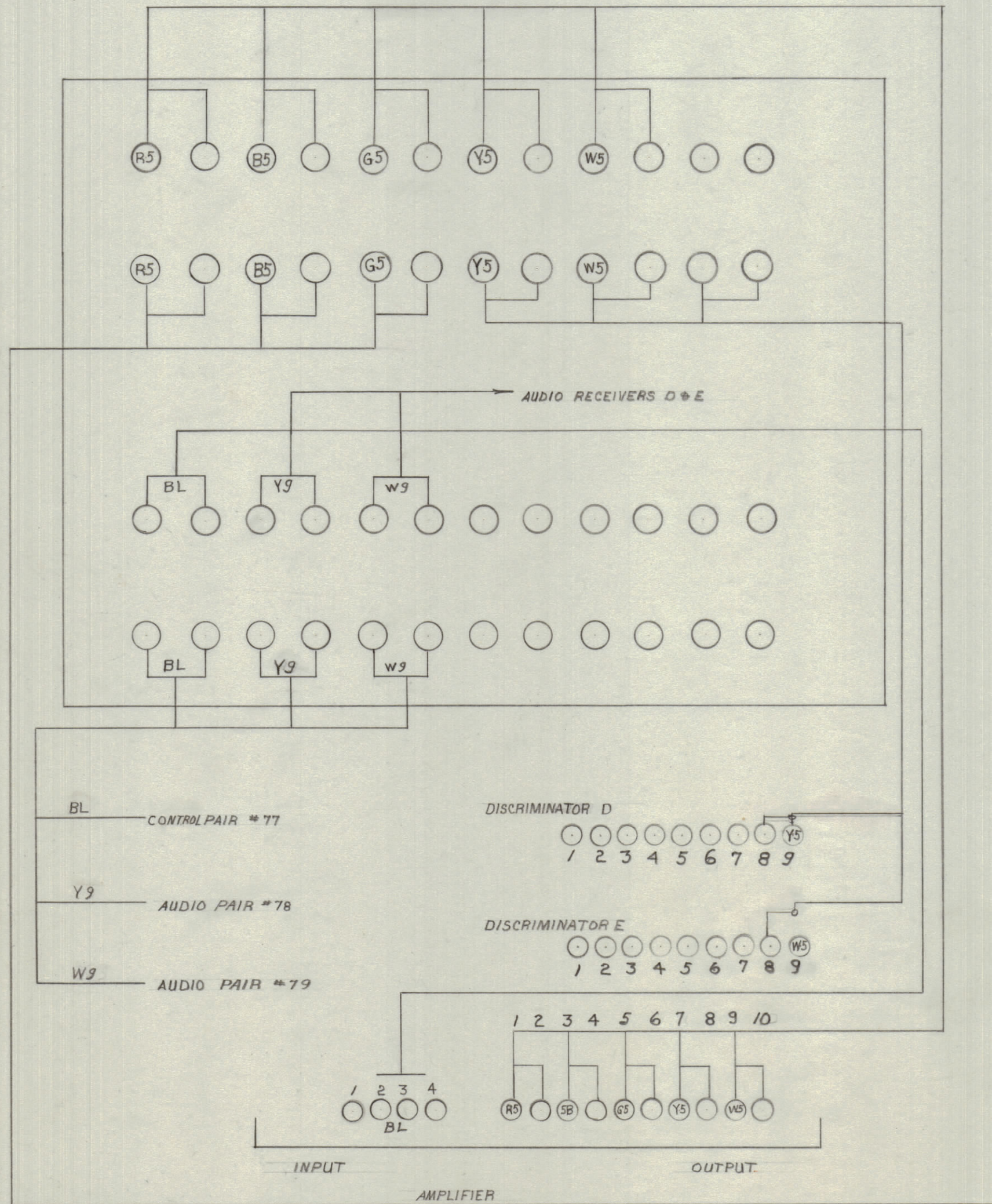
TERMINAL BOARD RACK NO.2
