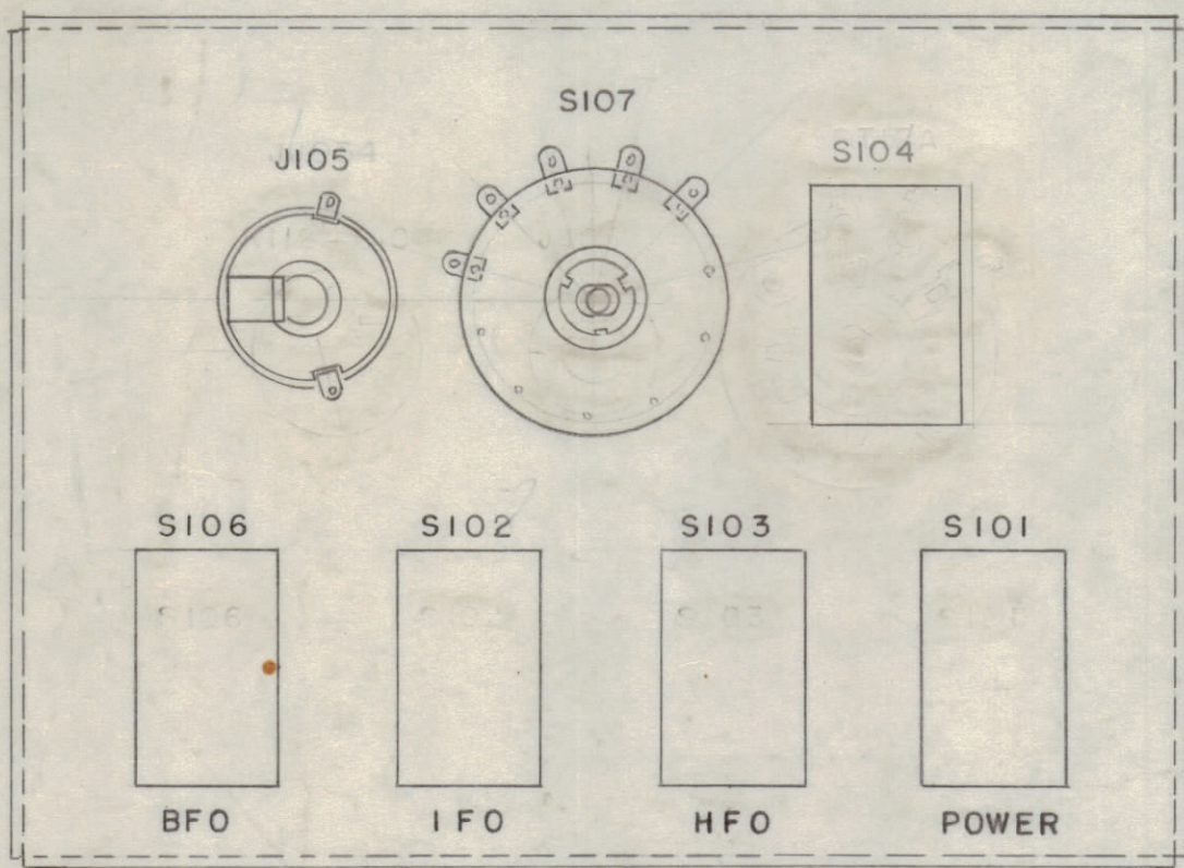
SUB-CONTROL PANEL REAR VIEW
