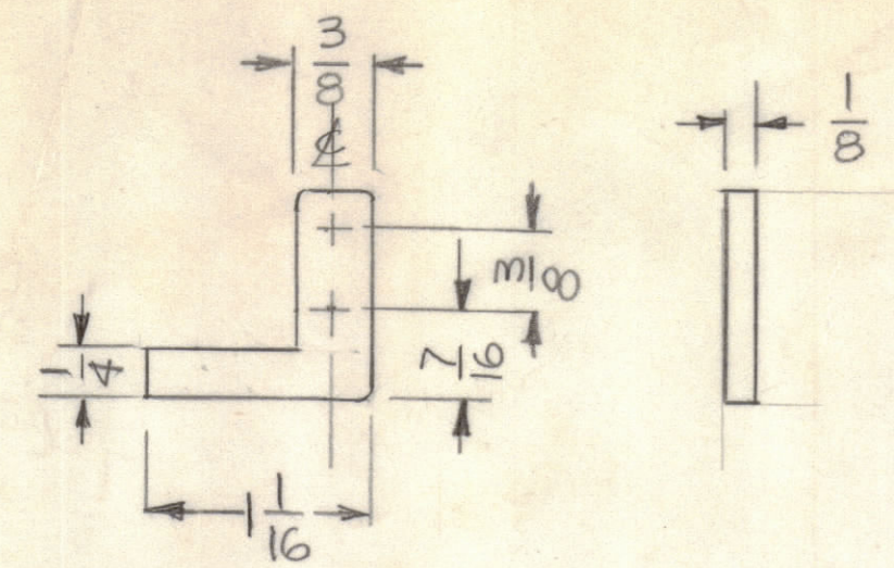
DETAIL C MATERIAL: BRASS
