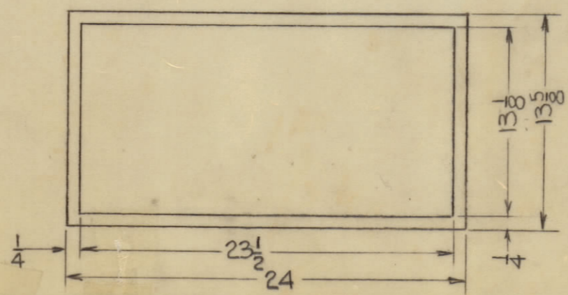
LAMINATING DETAIL MATL: VINYL PLASTIC, 015
