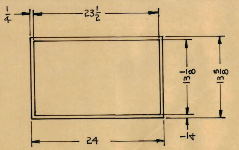
LAMINATING DETAIL MATERIAL: VINYL PLASTIC .015
