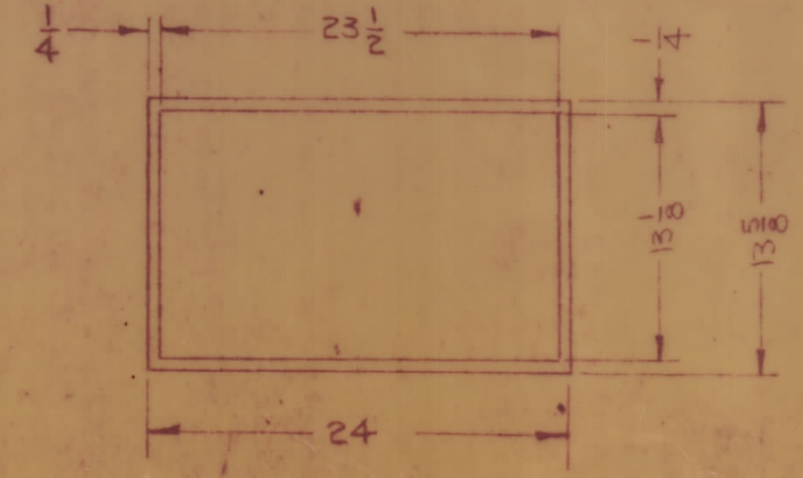
LAMINATING DETAIL MATERIAL: VINYL PLASTIC, .015
