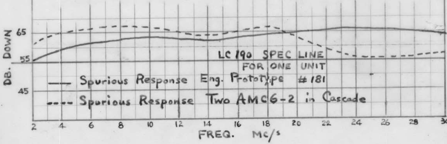
ELECTRICAL CHARACTERISTICS OF AMC6-2 WHEN OPERATED IN CASCADE
