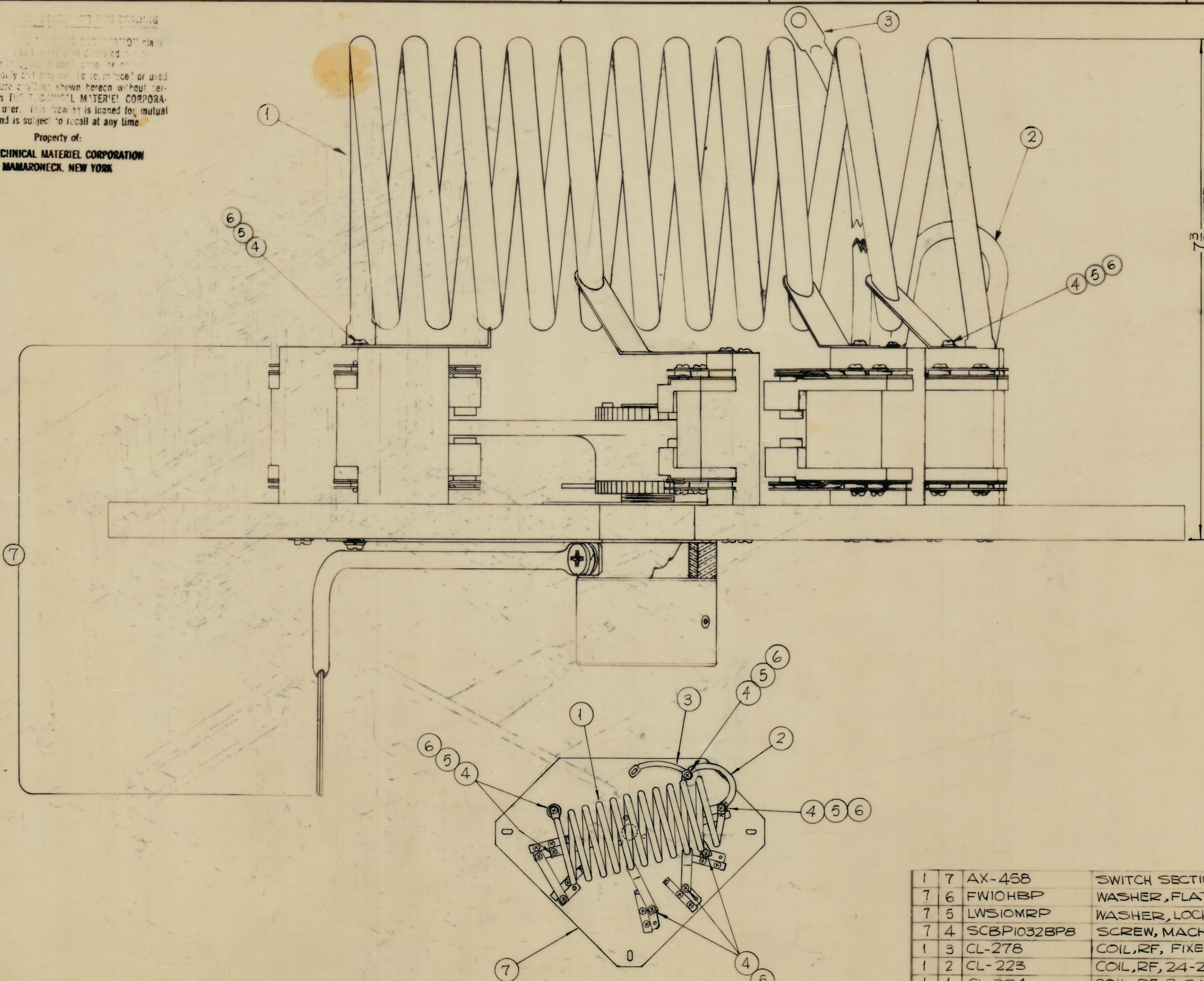
VIEW SHOWS POSITIONING OF POSTS AND COIL STRAPS.
