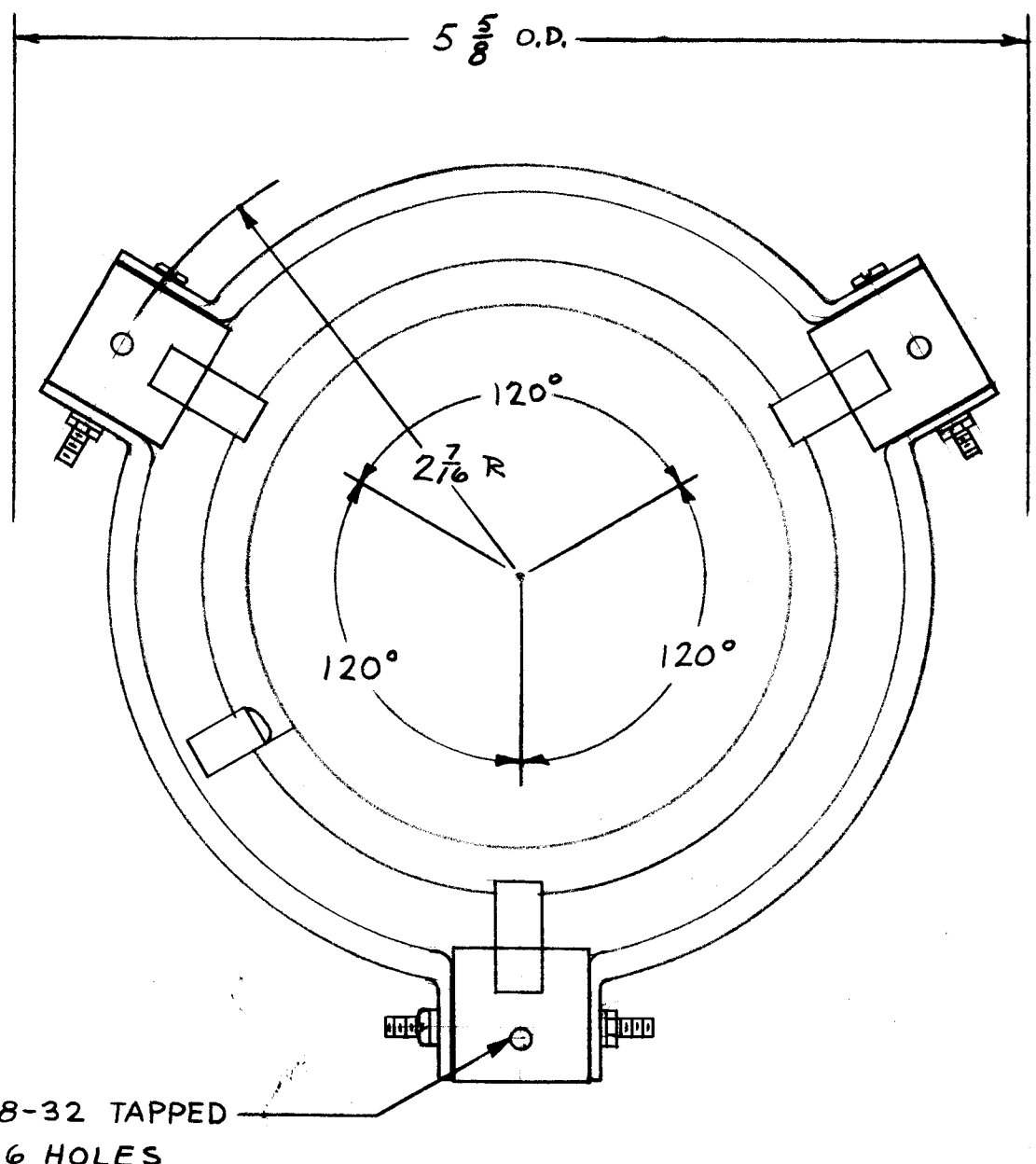
MOUNTING DETAIL
