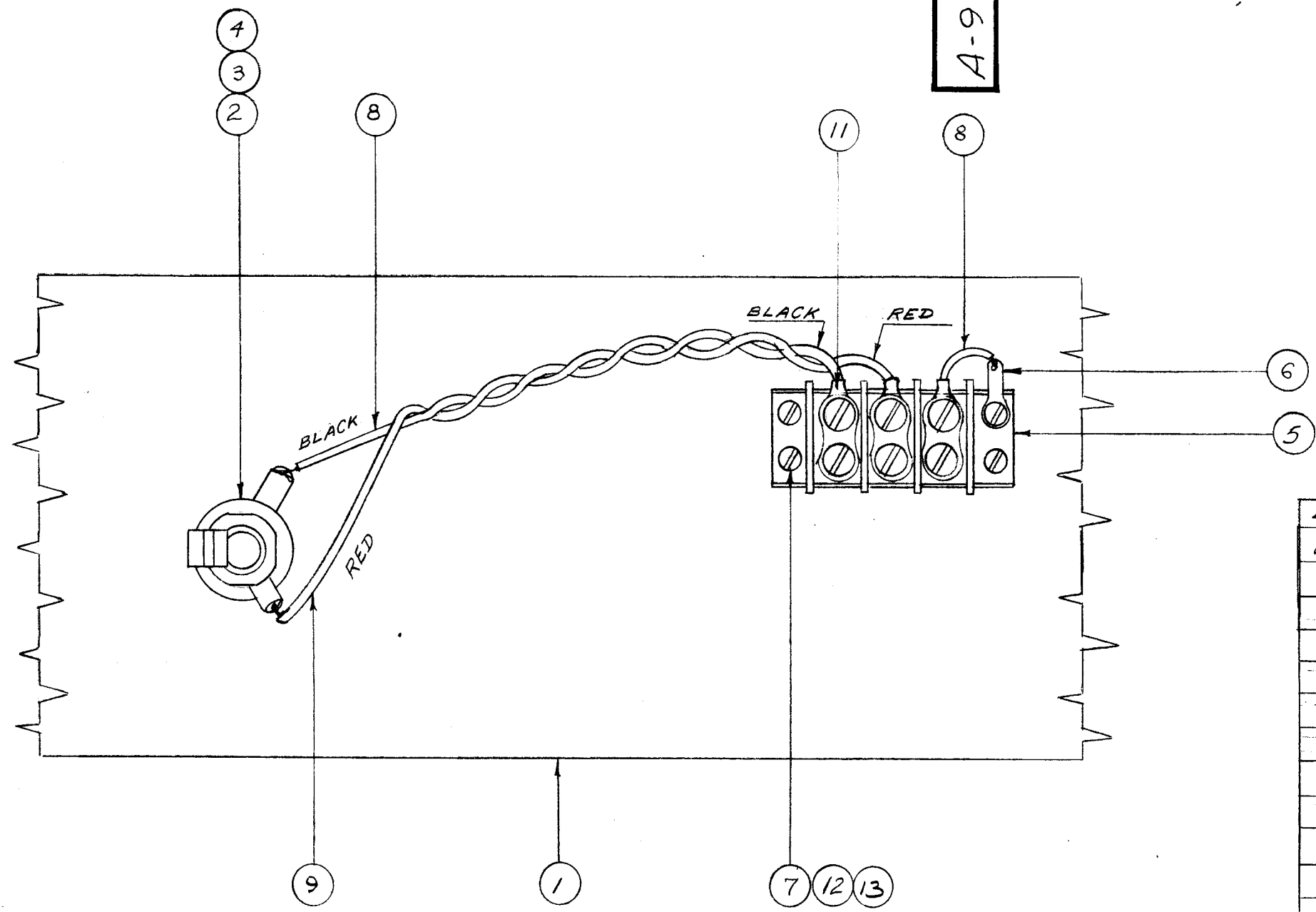
REAR VIEW OF FRONT PANEL SHOWN
