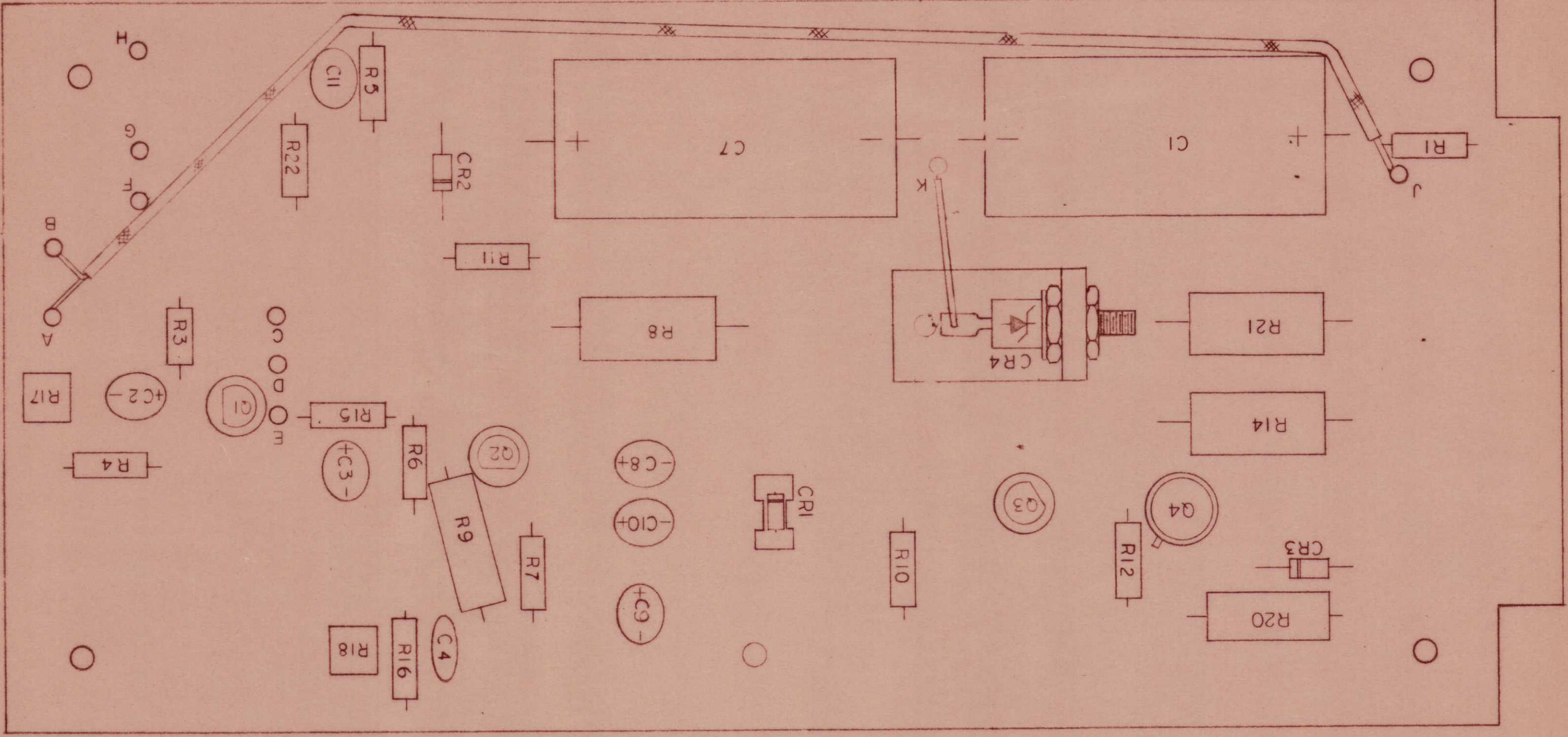
REFERENCE DRAWINGS - VIDEO PROCESSING AMPLIFIER CK 2105
