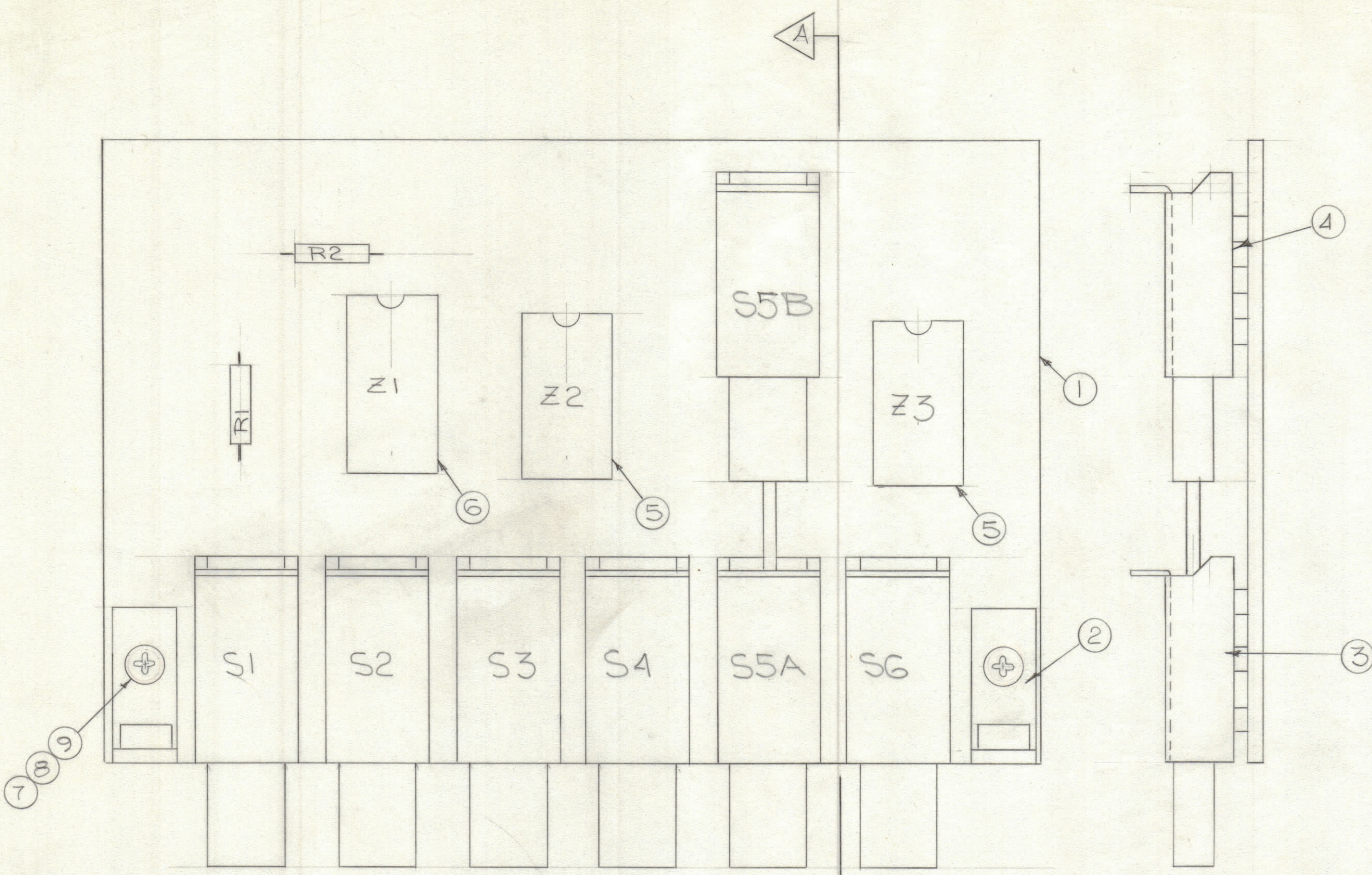
SECTION "A-A"
