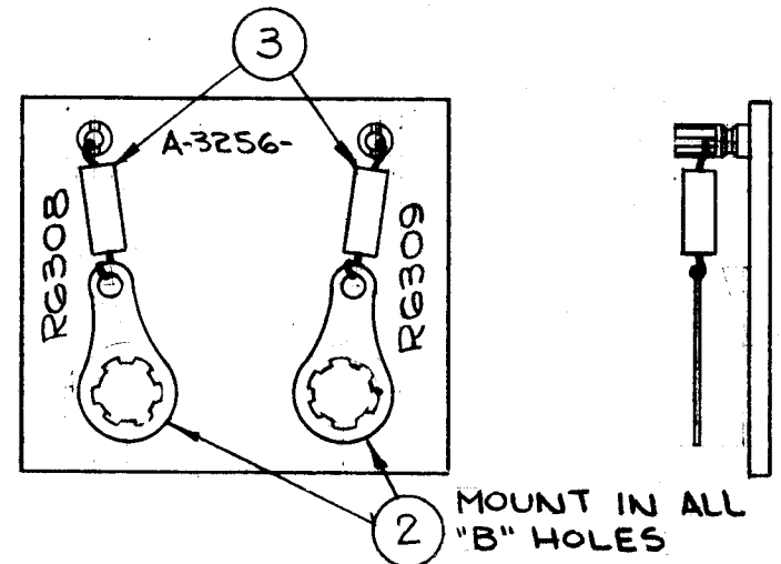
A-3256-4 FINAL ASSY
