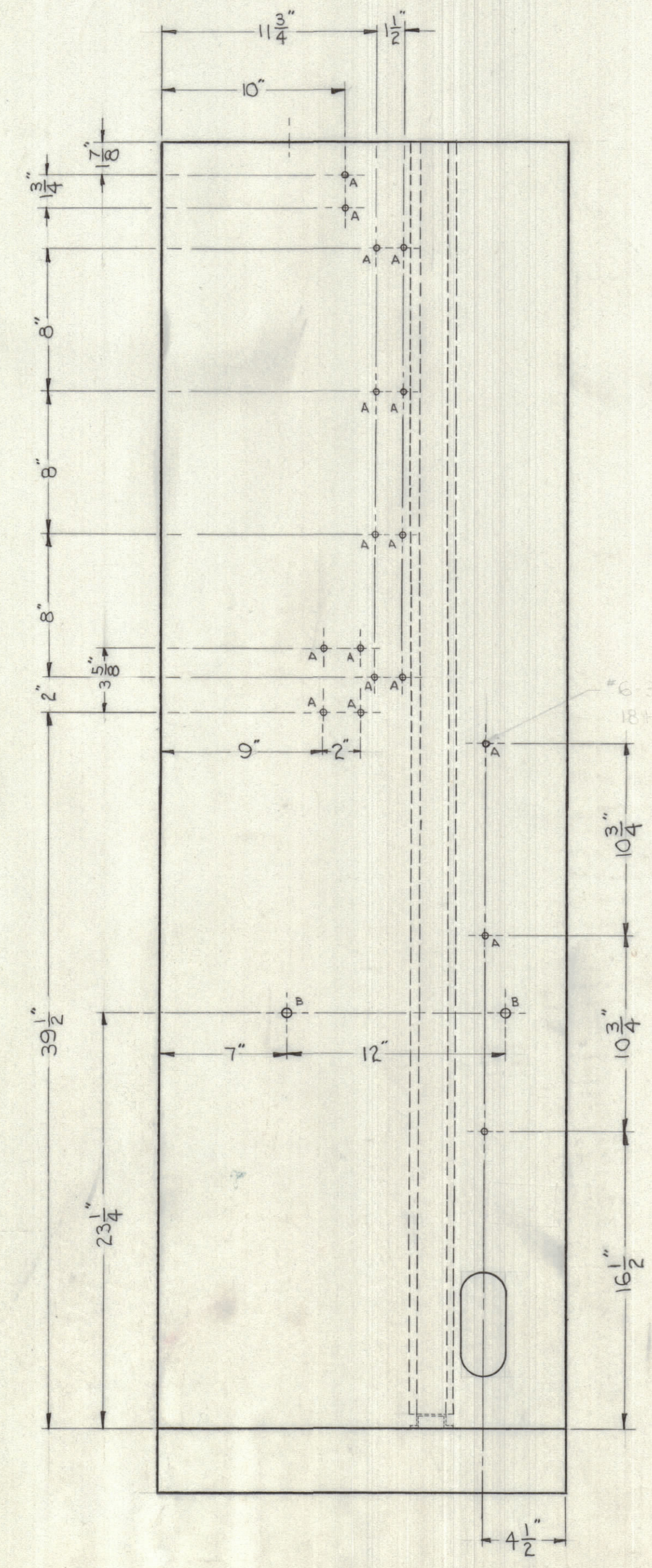
RIGHT SIDE VIEW
