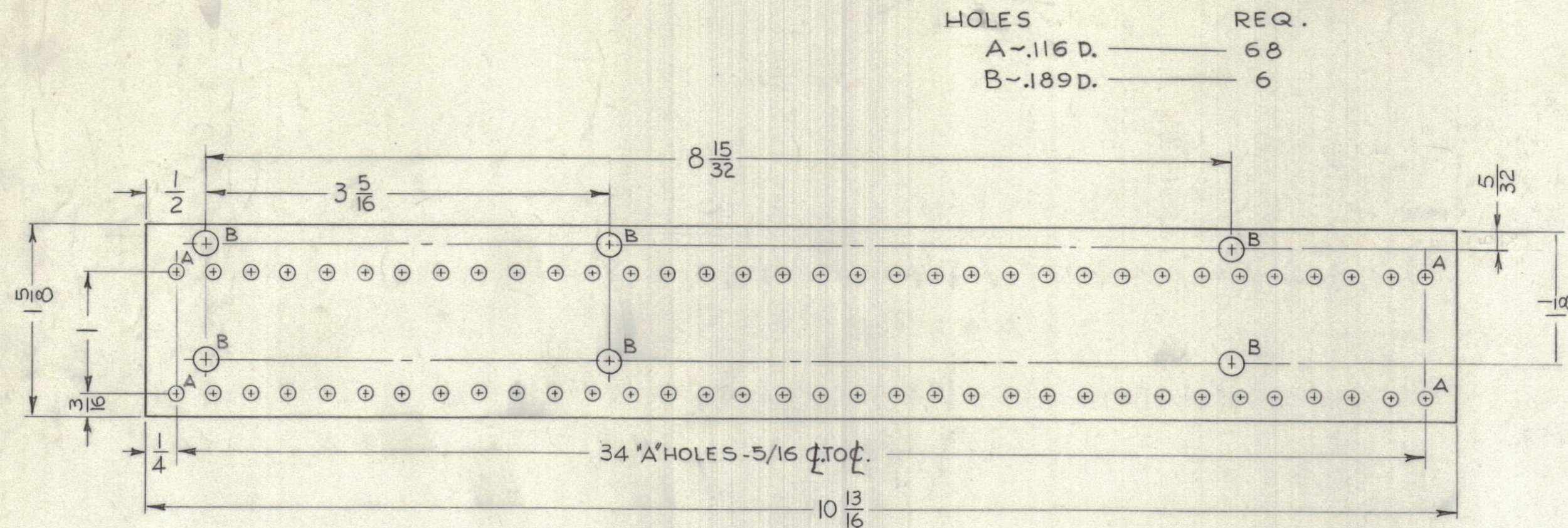
MACHINING - (A-2072-1) - MATERIAL PHENOLIC XXXP, 1/8" THK., FINISH NATURAL
