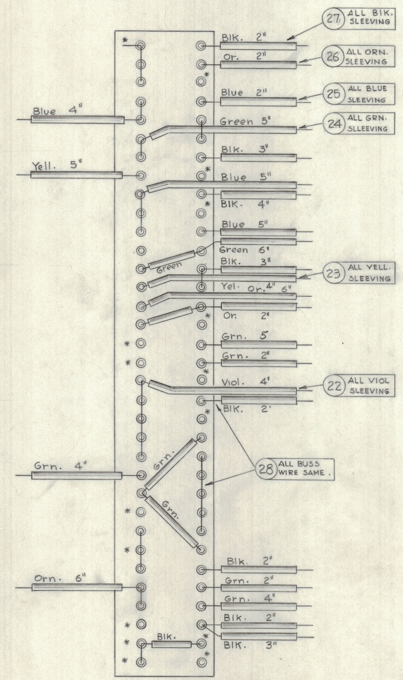
WIRING (A-2072-4) REAR NOTES - * DO NOT SOLDER THESE CONNECTIONS.
