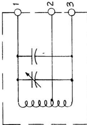
SCHMATIC
